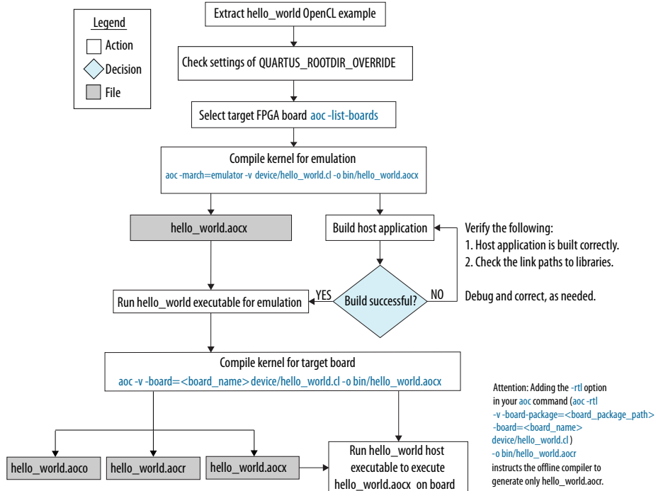
Figure 2. FPGA Programming Overview
