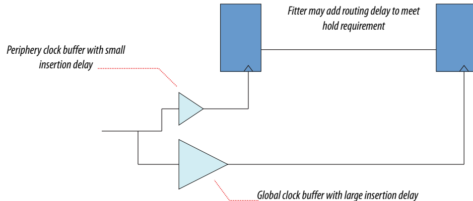
Figure 18. Clock Delay
