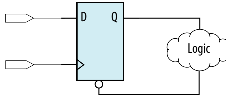
Figure 1. Combinational Loop Through Asynchronous Control Pin
