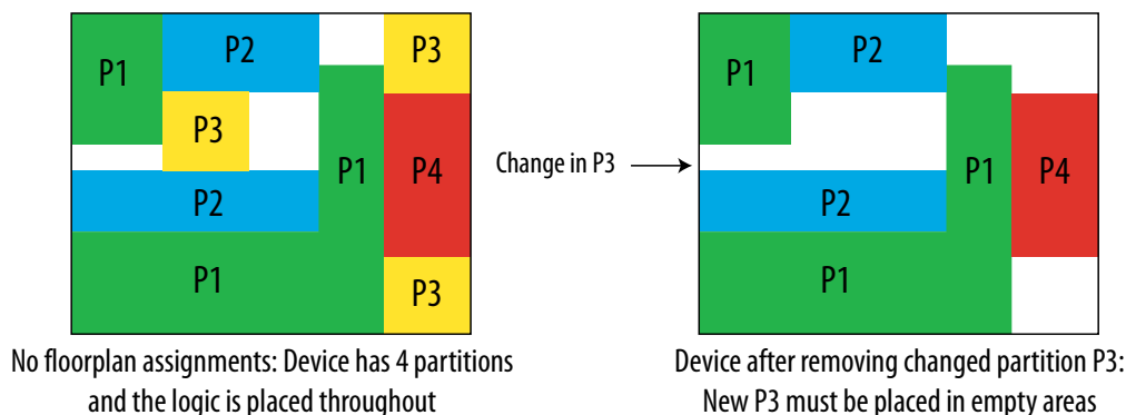
Figure 30. Representation of Device Floorplan without Location Assignments
