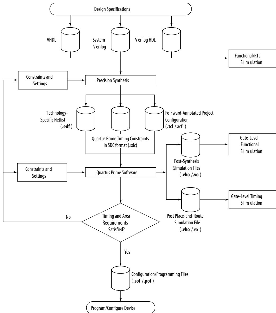
Figure 9. Design Flow Using the Precision Synthesis Software and Intel Quartus Prime Software
