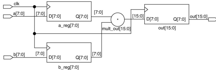
Figure 2. HDL Analyst View of LPM_MULT IP Core (Unsigned 8x8 Multiplier with Pipeline=2)
