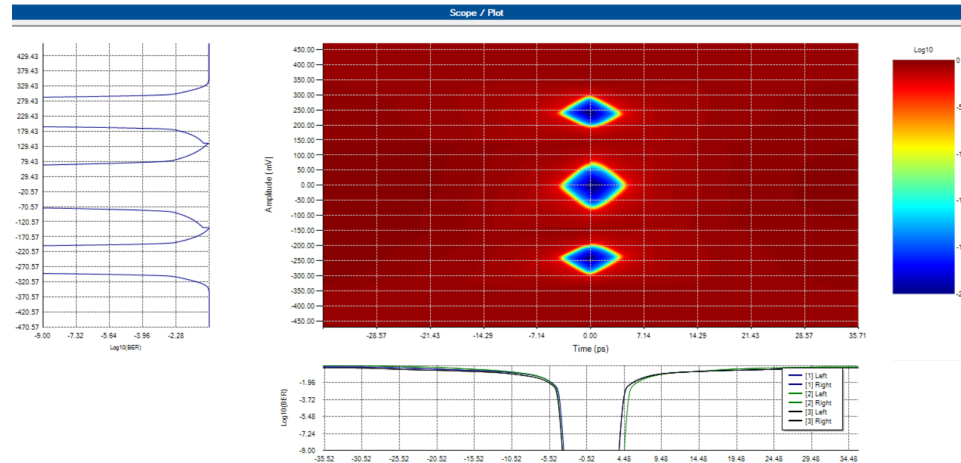
Figure 40. OIF Compliant Link Simulation Results: RX CDR FEC BER Eye
