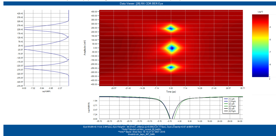
Figure 40. OIF Compliant Link Simulation Results: RX CDR FEC BER Eye
