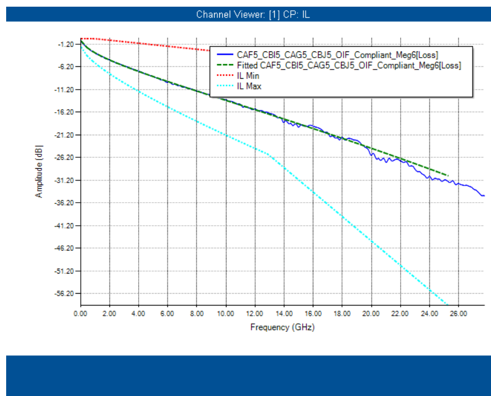
Figure 16. Megtron 6 Insertion Loss
