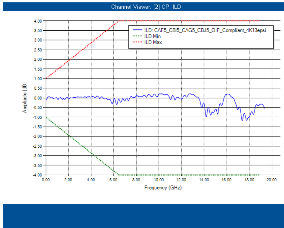
Figure 20. Nelco Insertion Loss Deviation
