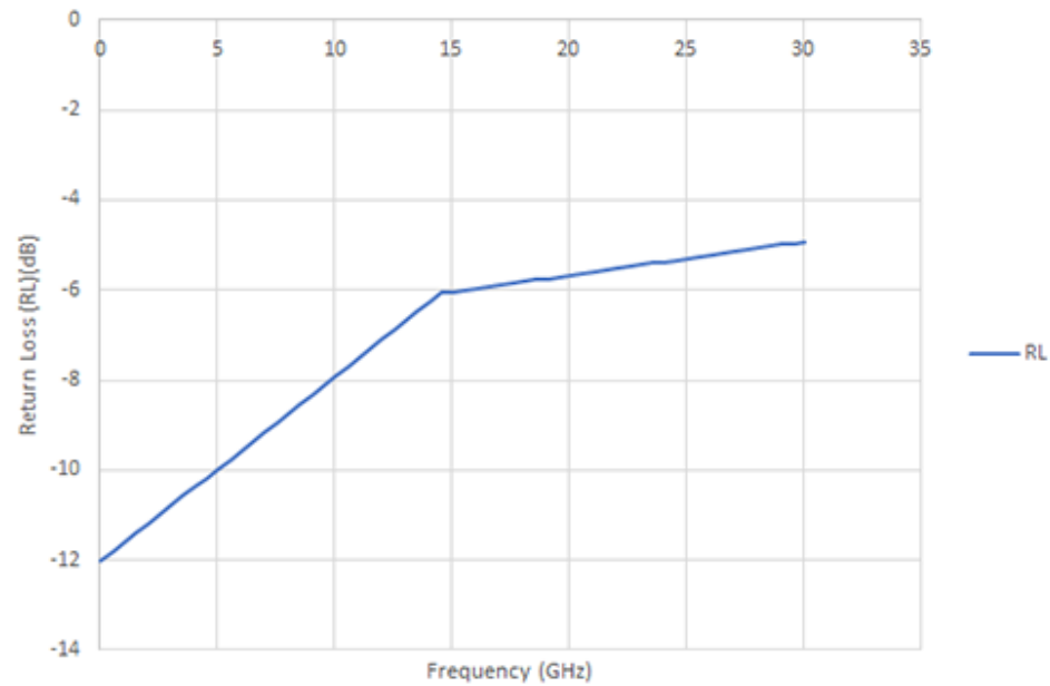
Figure 13. Transmitter Differential Return Loss Limit for 29 Gbaud/s (58 Gbps)
