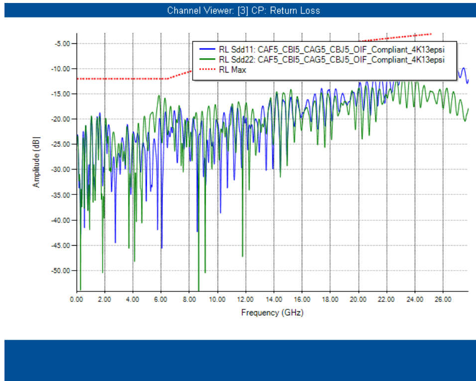
Figure 21. Nelco Return Loss
