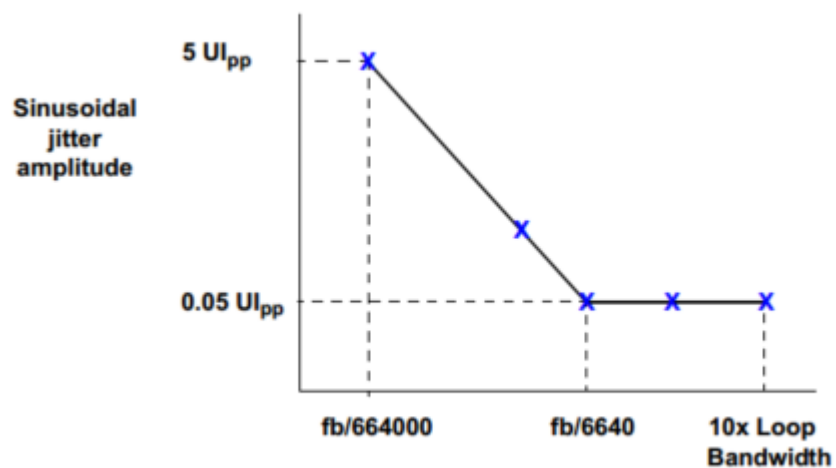
Figure 26. Receiver Jitter Tolerance Mask
