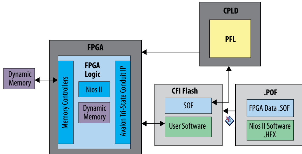
Figure 177. Nios II Application XIP from CFI Flash
