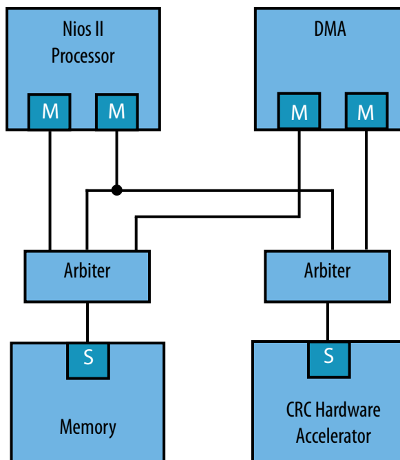
Figure 268. DMA and Hardware Accelerator for CRC
