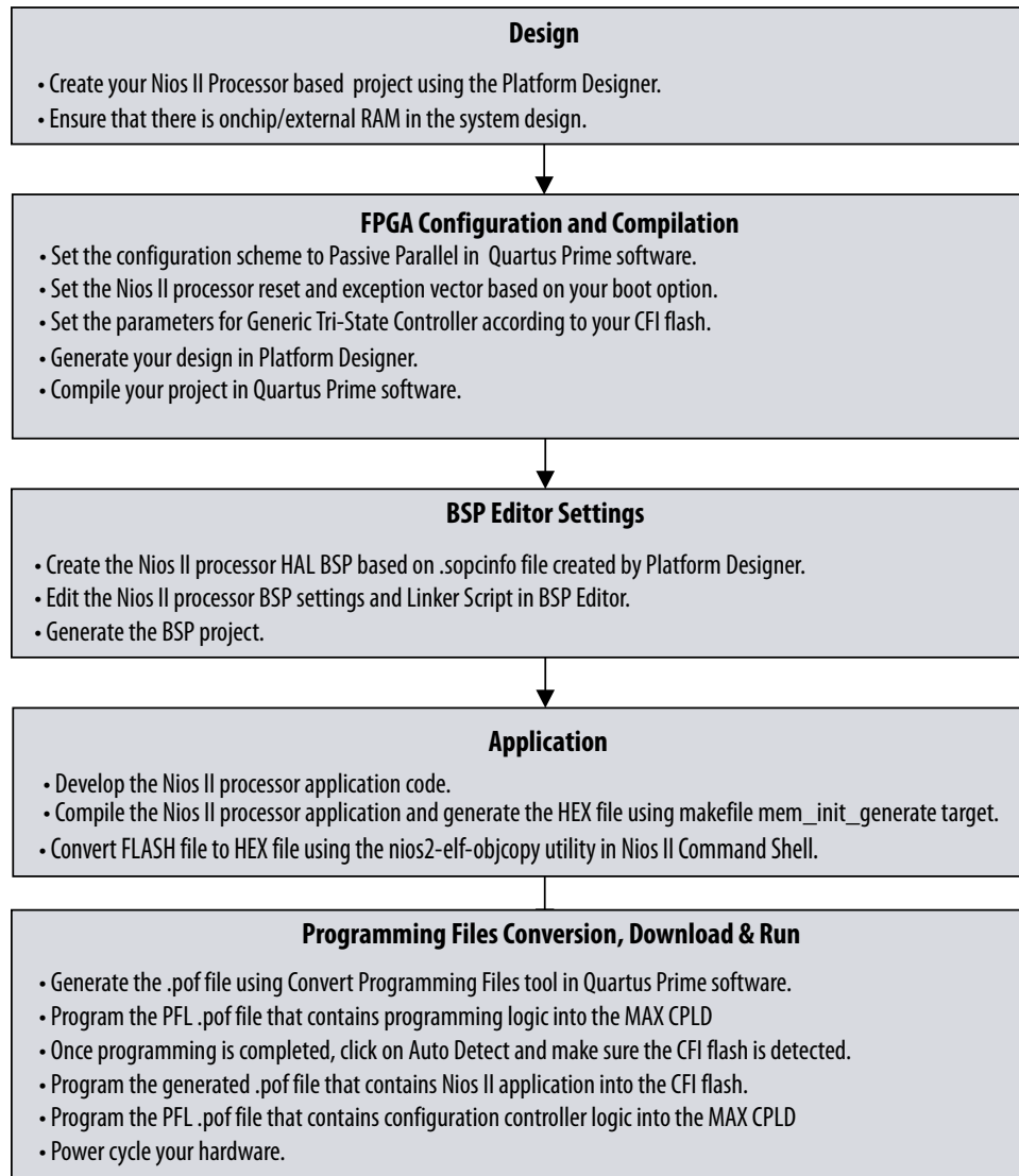
Figure 203. Design, Configuration and Booting Flow
