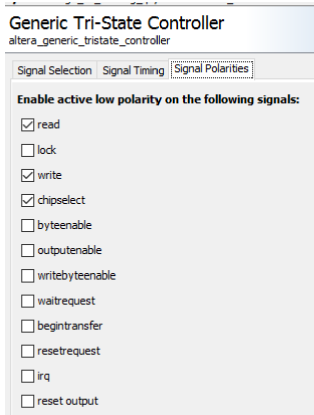
Figure 208. Signal Polarities
