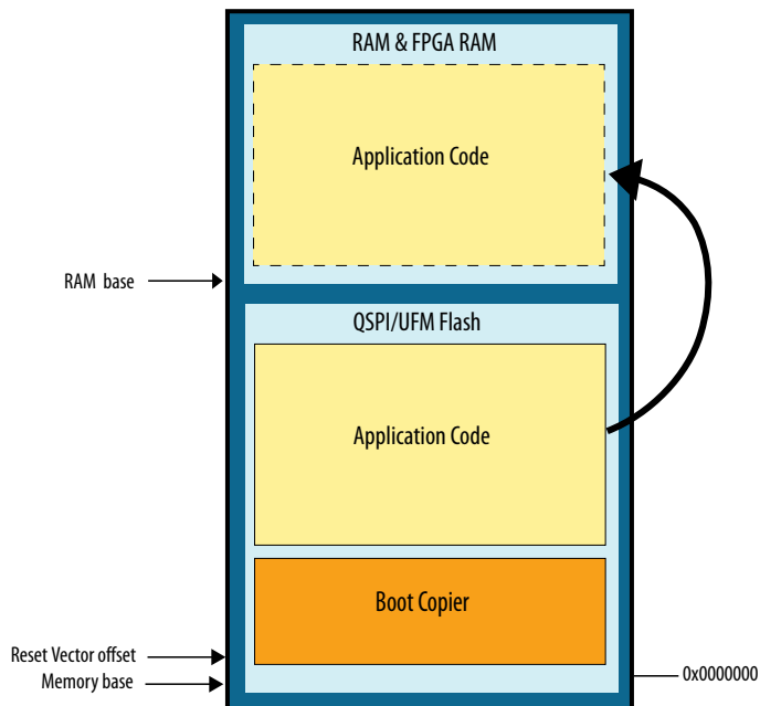
Figure 49. Memory Map of a System Using UFM with memcpy-based Boot Copier
