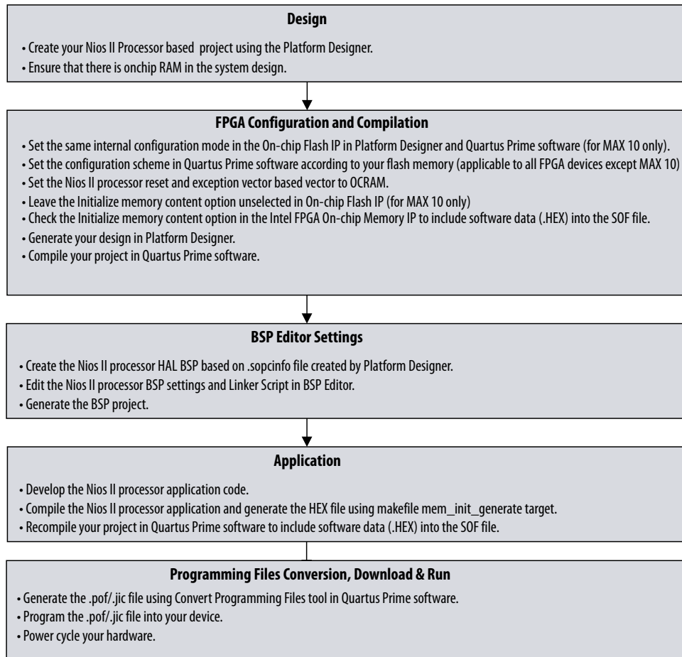
Figure 166. Configuration and Booting Flow
