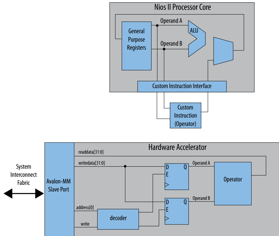
Figure 270. Implementation Differences between a Custom Instruction and Hardware Accelerator
