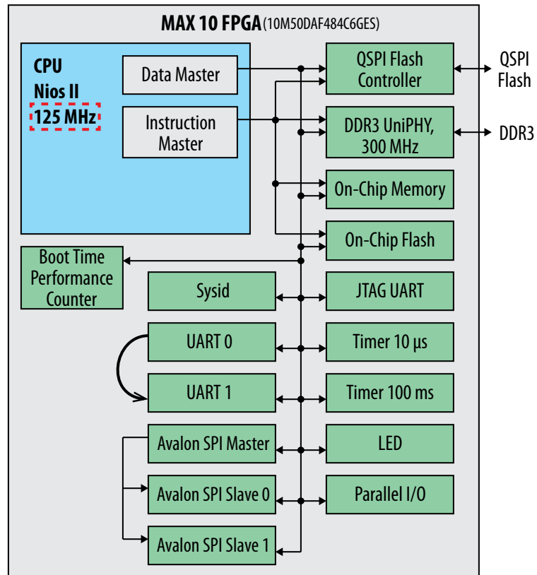
Figure 234. Nios II Design Block Diagram with Higher System Speed
