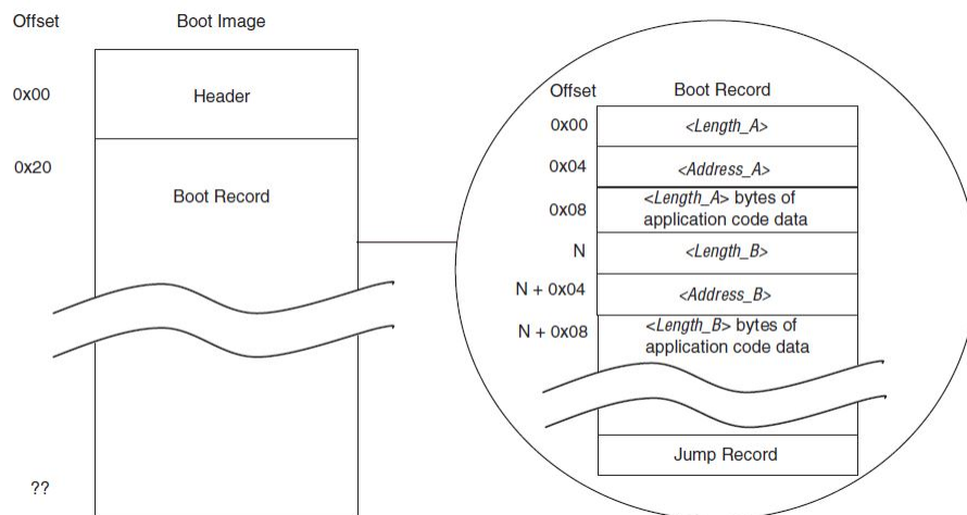
Figure 226. Example Boot Record Memory Map
