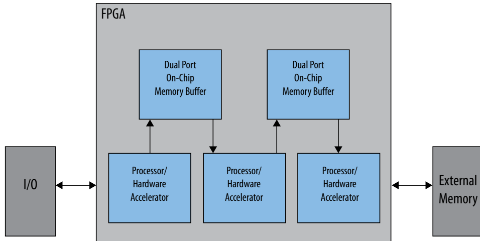
Figure 269. Using On-Chip Memory to Achieve High Performance
