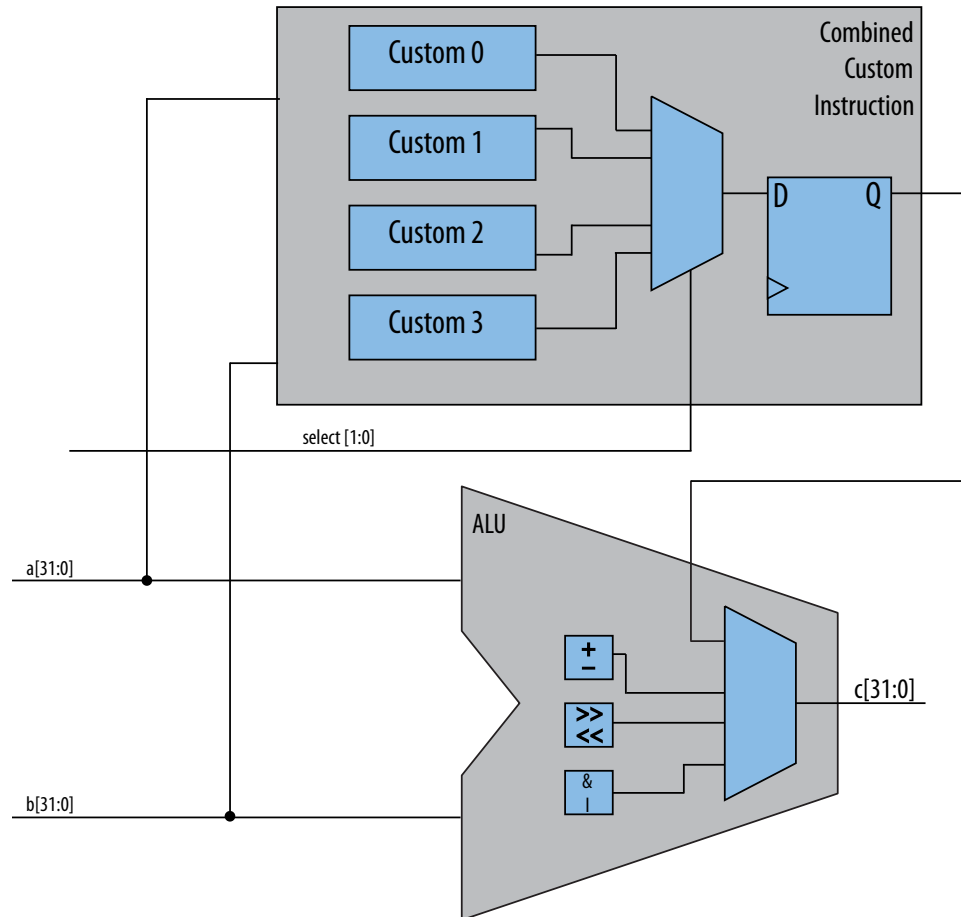
Figure 272. Combined Custom Instruction
