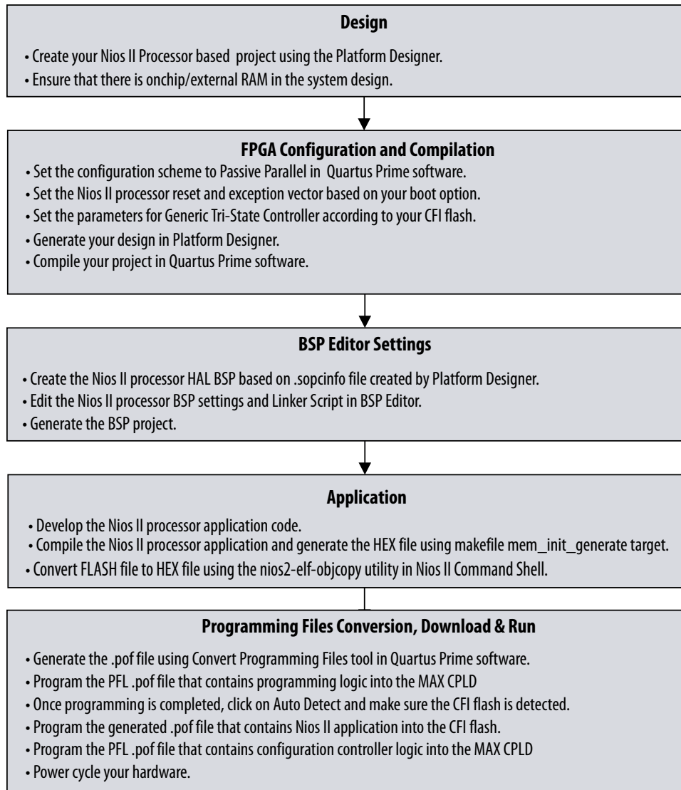
Figure 178. Design, Configuration and Booting Flow
