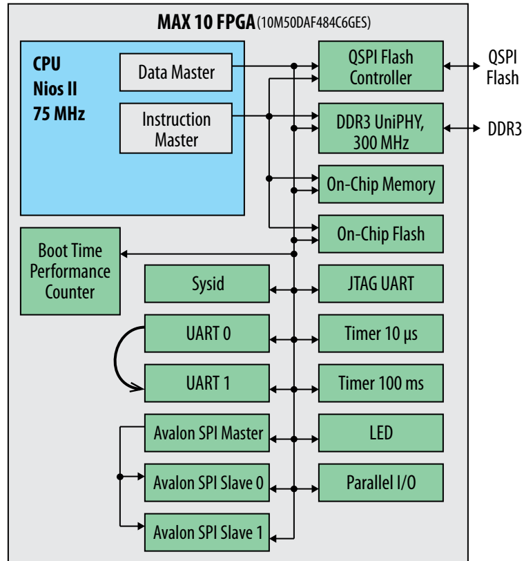
Figure 230. Boot Time Performance Analysis Design Block Diagram
