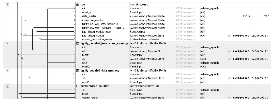
Figure 281. Connections for the Performance Counter
