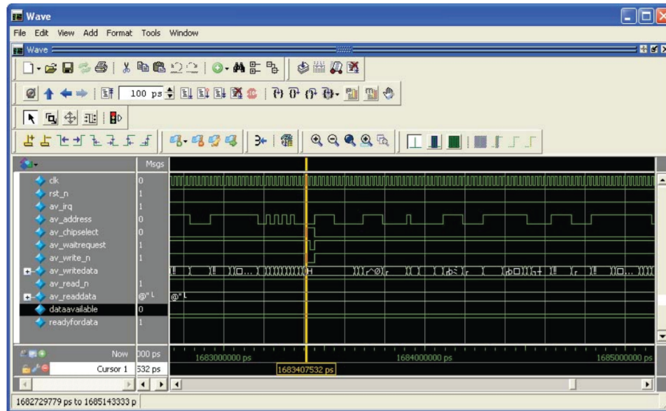
Figure 266. Simulation Results
