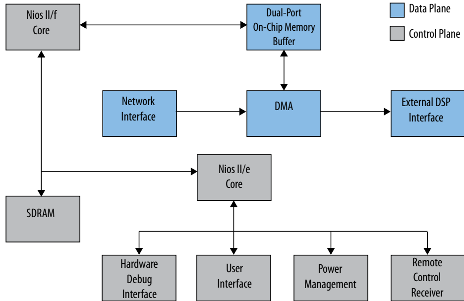
Figure 275. High Performance Video System
