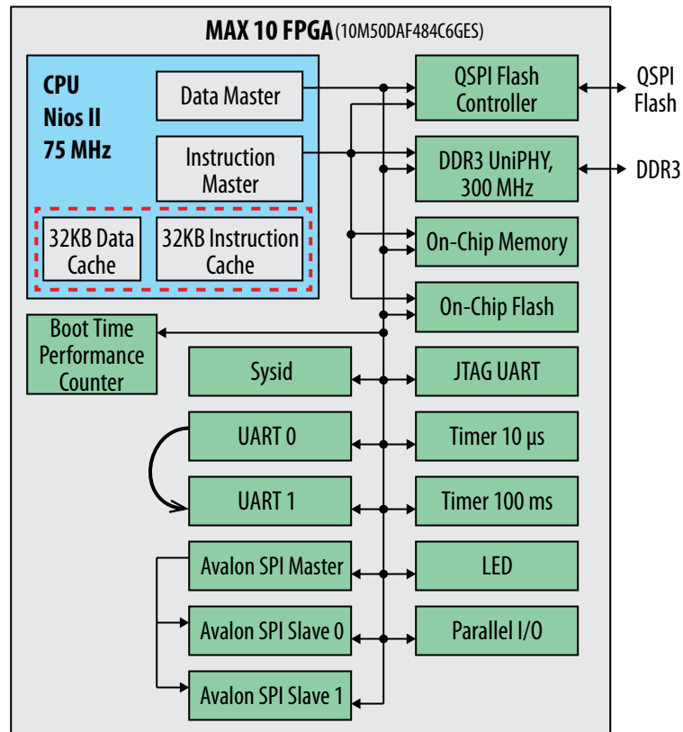
Figure 233. Nios II Design Block Diagram with Processor Caches Enabled
