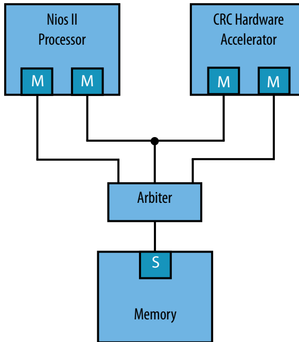
Figure 267. A Hardware Accelerator for CRC
