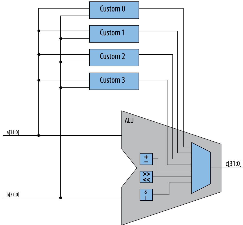
Figure 271. Individual Custom Instructions
