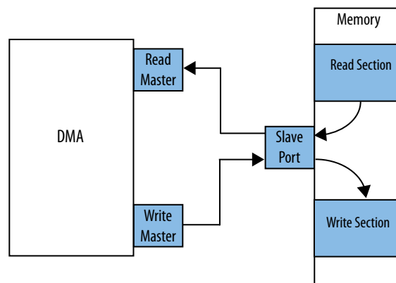
Figure 263. Using a DMA to Stress Test Memory Devices
