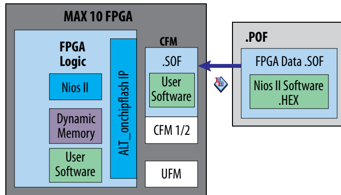
Figure 165. Nios II Application XIP from OCRAM in FPGA Device Configured from Flash Memory
