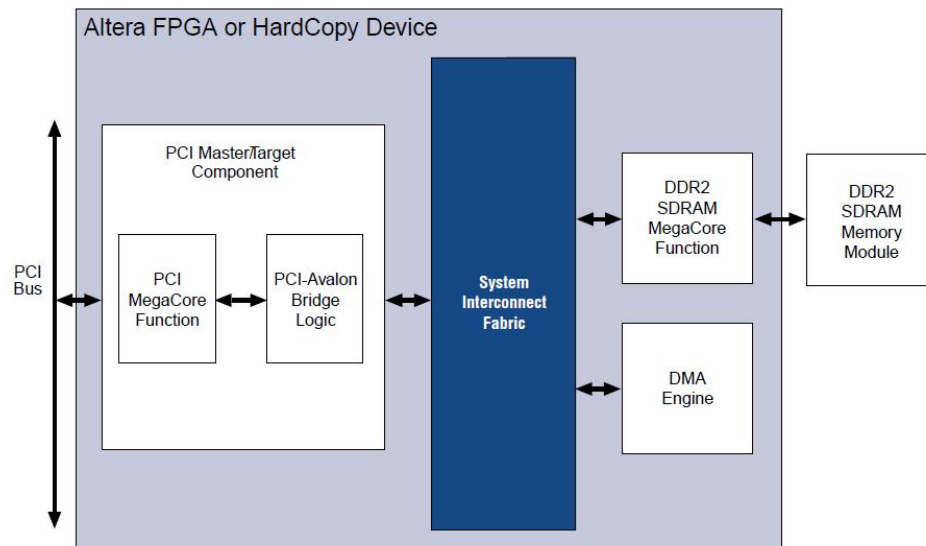
Figure 10. PCI Intel FPGA IP Function in a Platform Designer System
