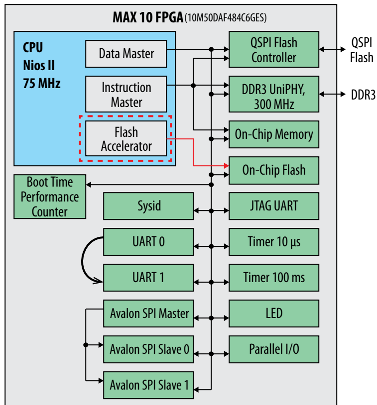
Figure 235. Nios II Design Block Diagram with Flash Accelerator Enabled
