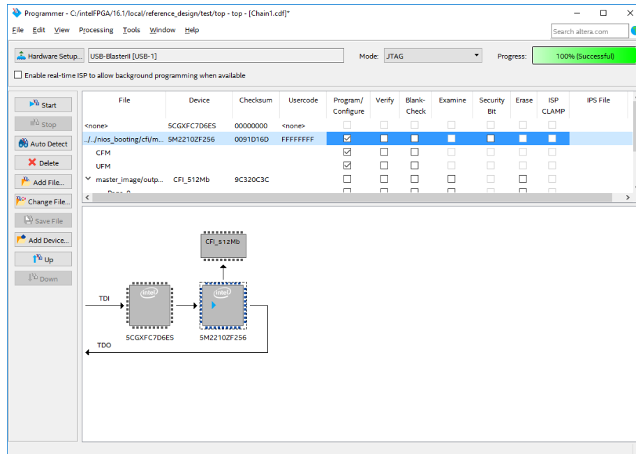
Figure 224. Program MAX CPLD with Configuration Controller Logic
