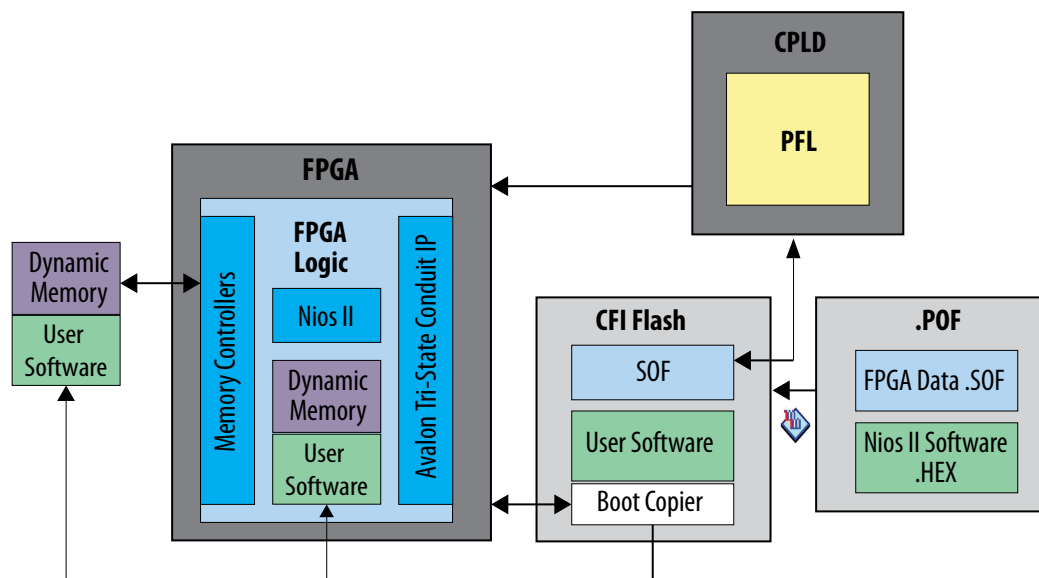
Figure 202. Nios II Application Copied from CFI Flash to RAM using Boot Copier
