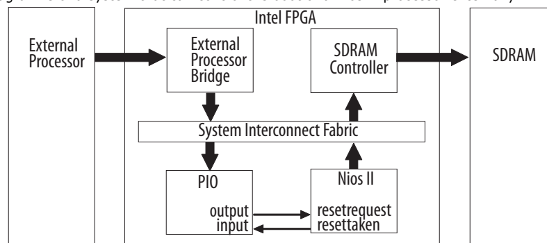
Figure 229. Block Diagram of Externally Controlled Nios II Boot System
