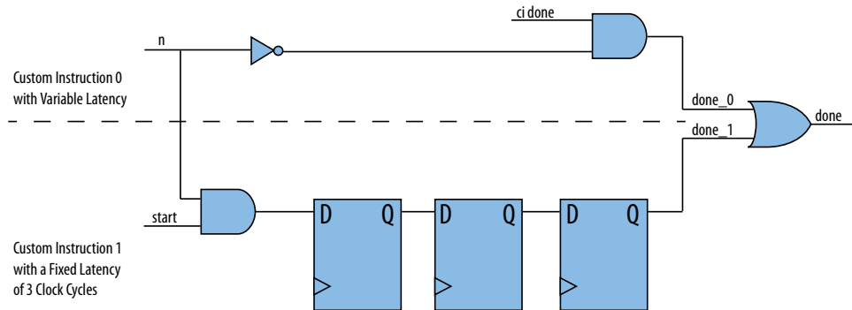
Figure 273. Sequencing Logic for Mixed Latency Combined Custom Instruction
