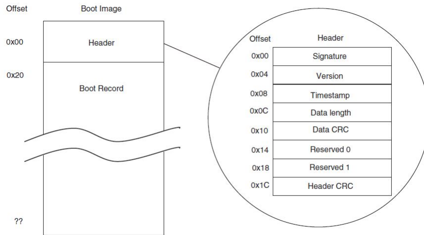
Figure 225. Example Boot Image Format
