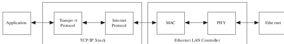
Figure 278. The Ethernet System Hierarchy
