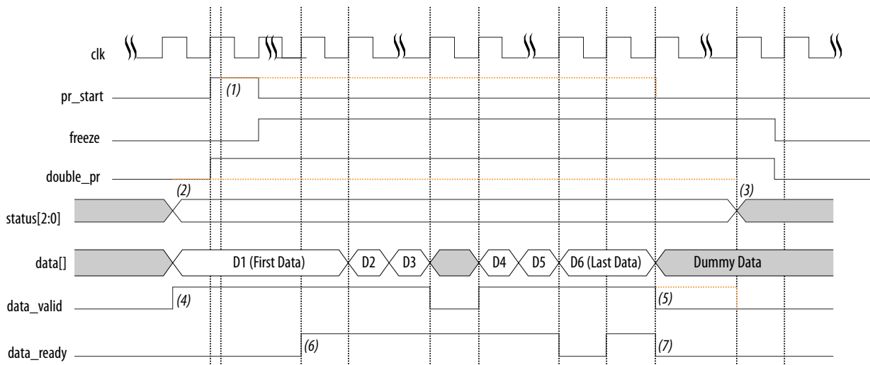
Figure 7: Partial Reconfiguration Timing
