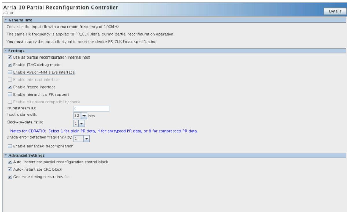
Figure 4: Partial Reconfiguration IP Core in the IP Catalog
