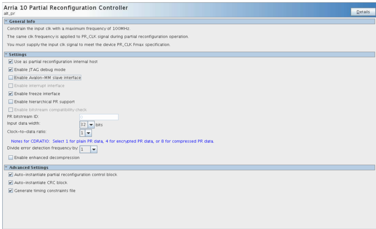
Figure 3: Partial Reconfiguration IP Core in the Qsys Interface
