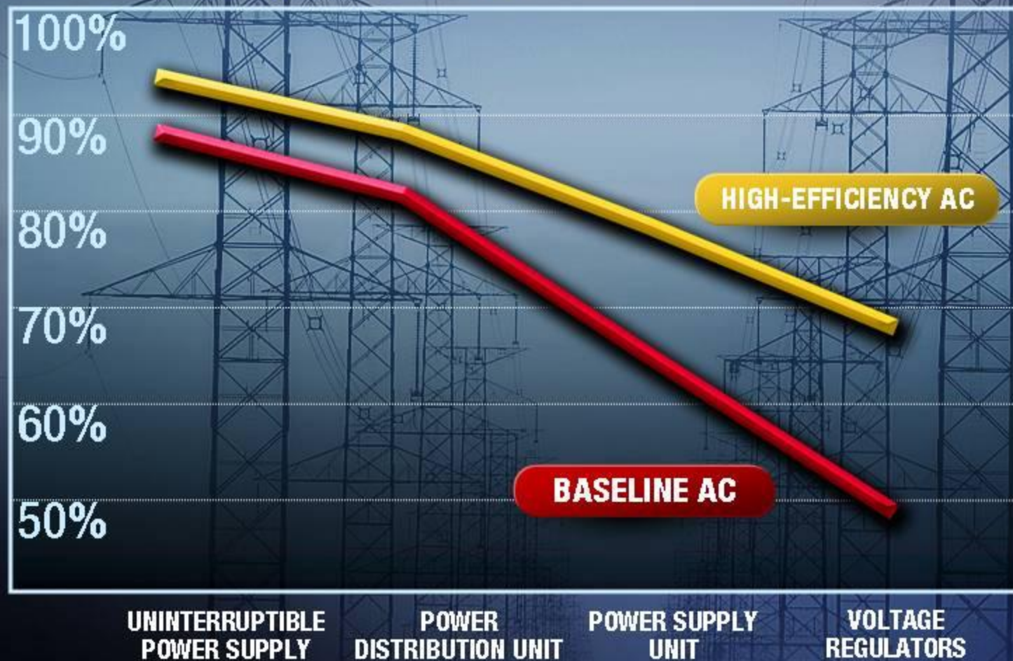
CUMULATIVE DATACENTER POWER DELIVERY EFFICIENCY
