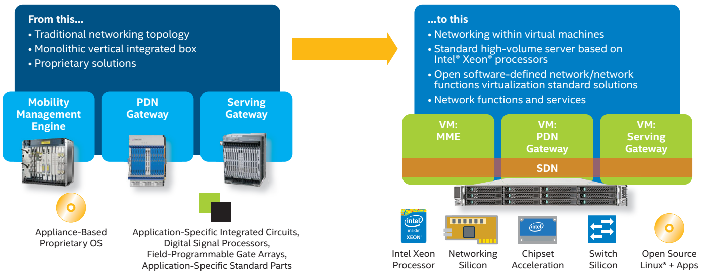
Figure 2. Virtualizing network functions enables service providers to eliminate expensive purpose-built devices and consolidate functions on more economical standard high-volume servers
