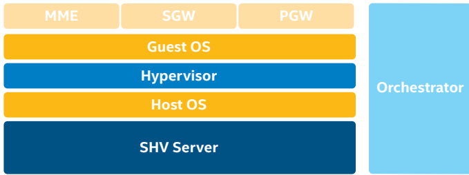
Figure 3. A vEPC solution virtualizes EPC functions—including Mobility Management Entity, Serving Gateway, and Packet Data Network Gateway—on a standard high-volume server powered by Intel® technologies.
