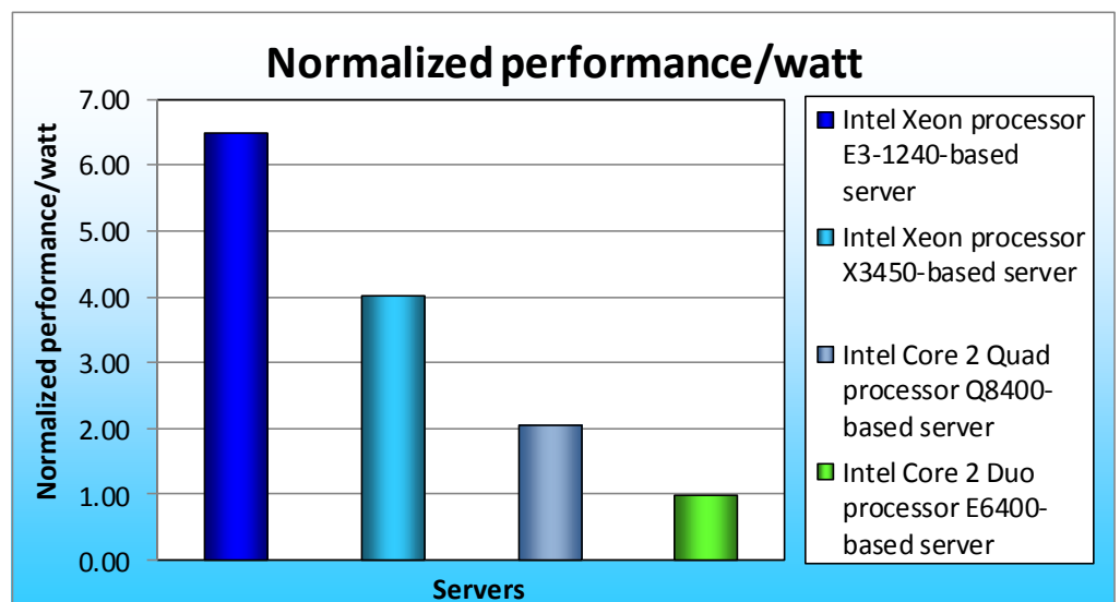
Figure 2: Normalized performance-per-watt results of the Intel processor-based servers across the three benchmarks relative to the Intel Core 2 Duo processor E6400-based server. Higher numbers are better.
