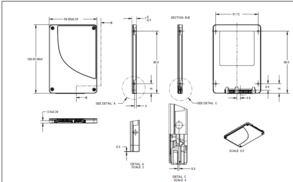
Figure 1. Intel SSD DC S3700 Series, 2.5-inch Form Factor Dimensions
