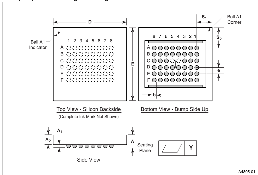
Figure 15-3. Example \mu BGA* Package Drawing and Dimensions
