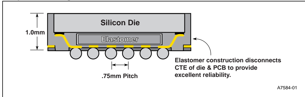
Figure 15-2. The \mu BGA* Package
