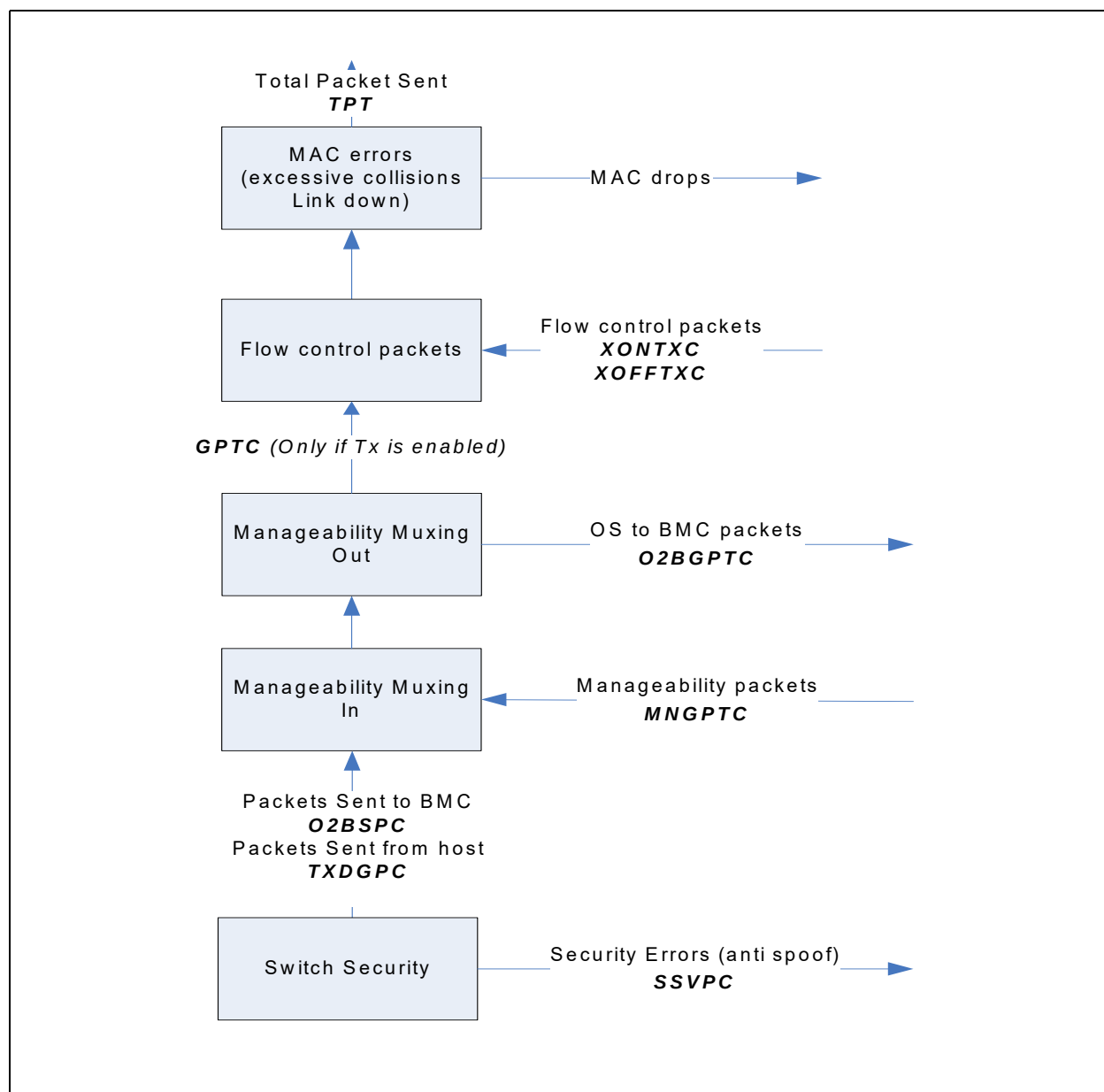
Figure 6.21. Transmit Flow Statistics
