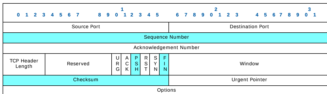
Figure A.5. TCP Header (Traditional Representation)
