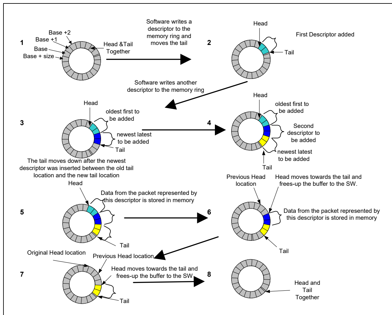
Figure 6.11. Descriptors and Memory Rings
