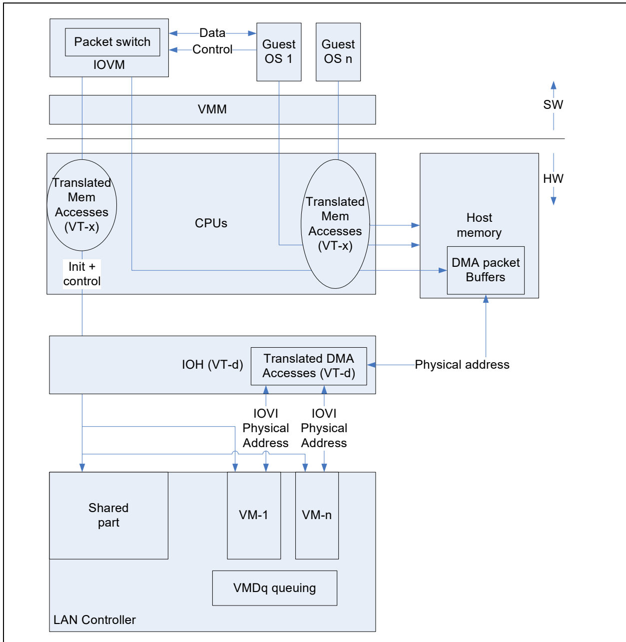
Figure 6.32. System Configuration for VMDq2 Mode
