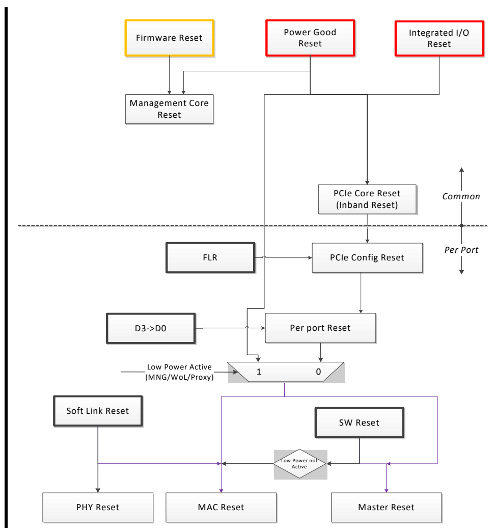
Figure 3.1. Reset Tree
