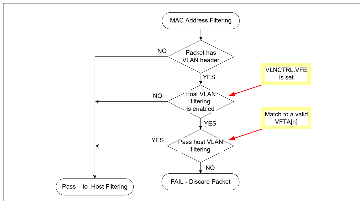
Figure 6.3. VLAN Filtering
