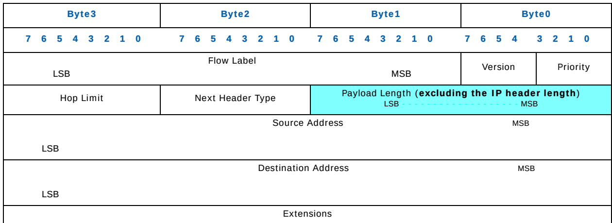
Figure A.4. IPv6 Header (Little Endian Order - byte 0 first on the wire)
