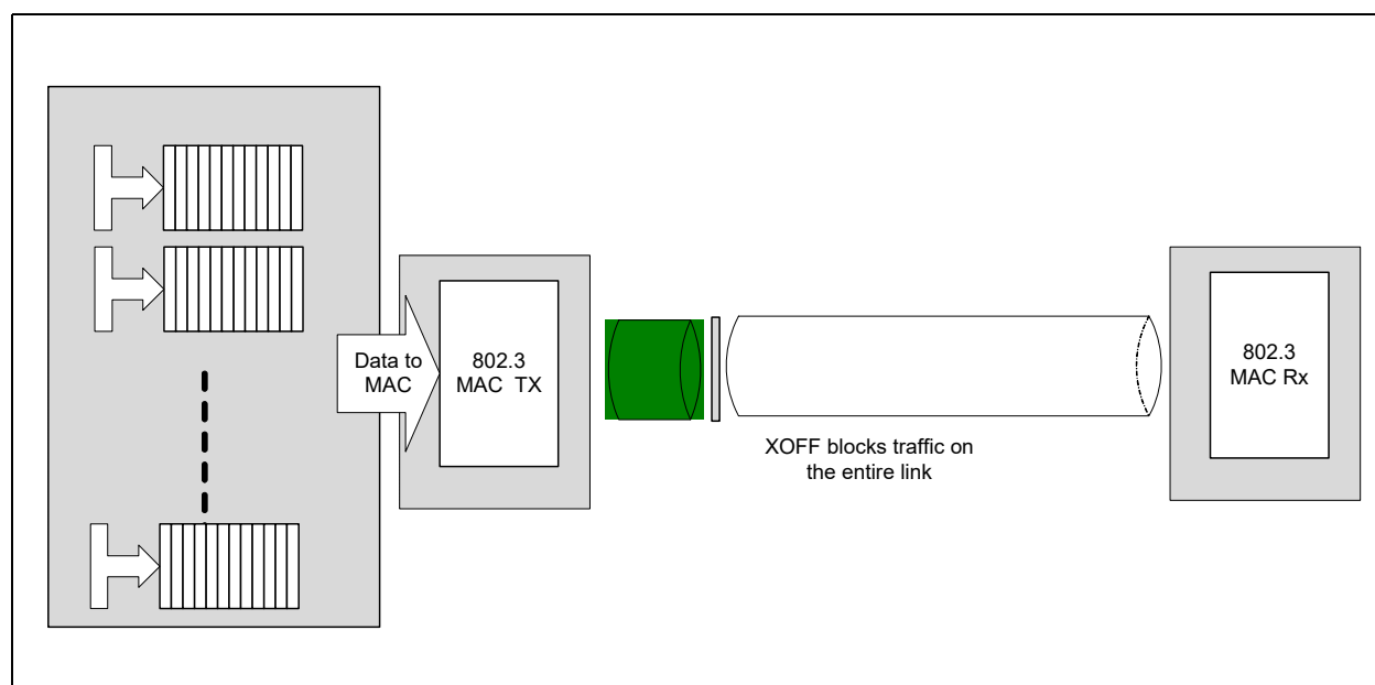
Figure 2.13. 802.3X Link Flow Control (PAUSE)
