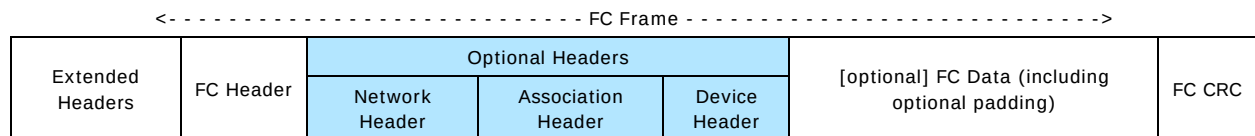
Figure A.13. FC Frame format with Optional Headers (without ESP Header)
