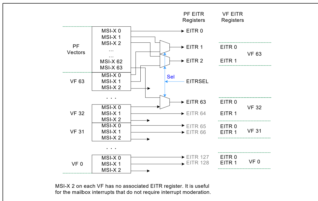
Figure 6.29. PF / VF MSI-X Vectors Mapping to EITR
