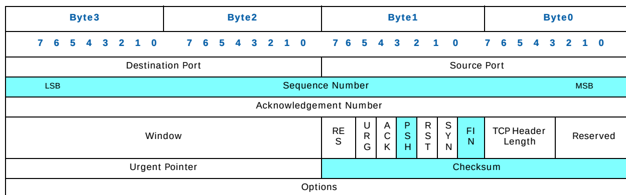
Figure A.6. TCP Header (Little Endian)
