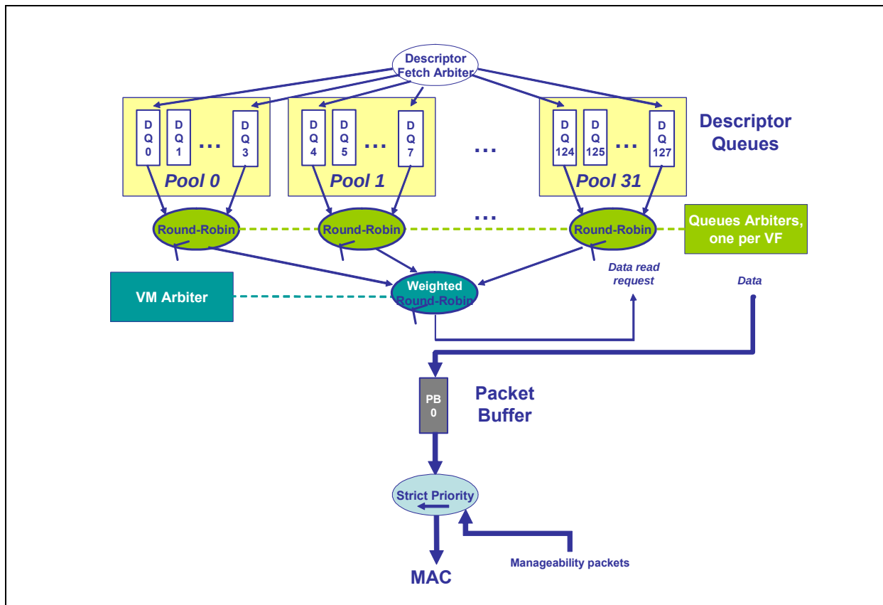
Figure 6.18. Transmit Architecture VT-on — 32 VFs
