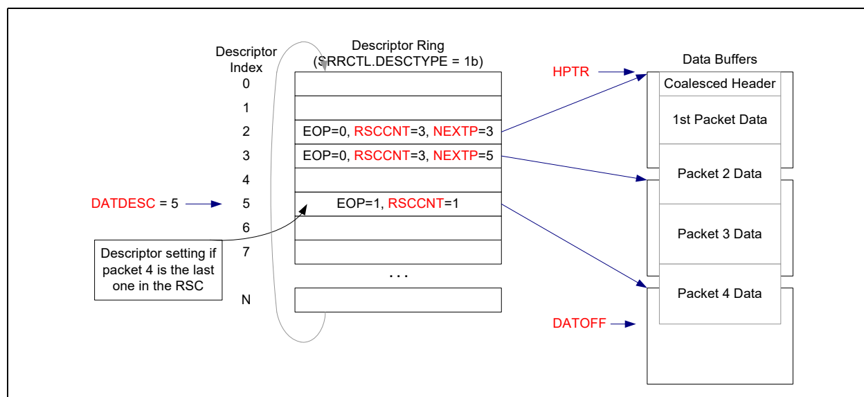
Figure 6.36. RSC Functionality (No Header Split)
