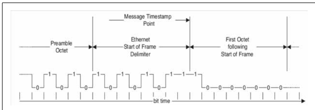
Figure 6.31. Time Stamp Point
