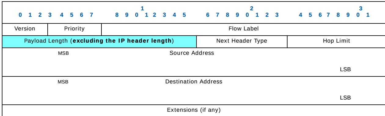
Figure A.3. IPv6 Header (Traditional Representation - most left byte first on the wire)
