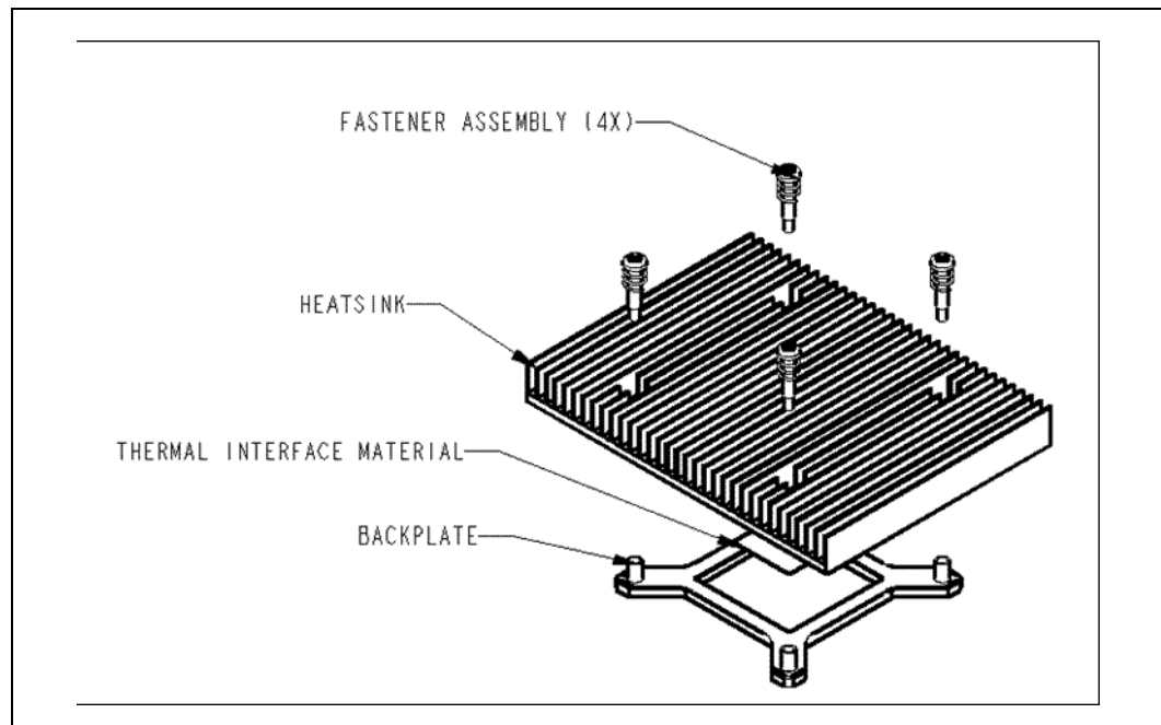
Figure 14. CompactPCI Reference Heatsink Assembly
