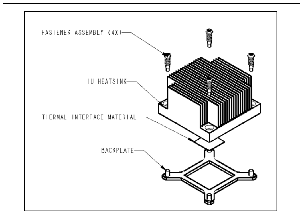
Figure 12. 1U Reference Heatsink Assembly
