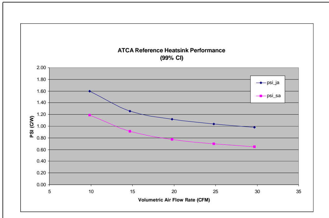
Figure 11. AdvancedTCA* Heatsink Thermal Performance vs. Volumetric Airflow Rate
