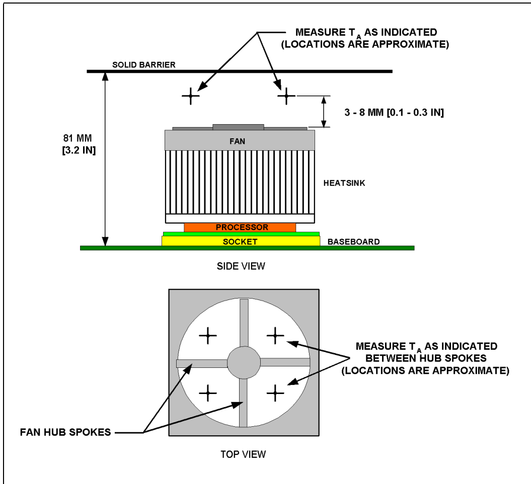
Figure 17. Measuring T_{LA} with an Active Heatsink
