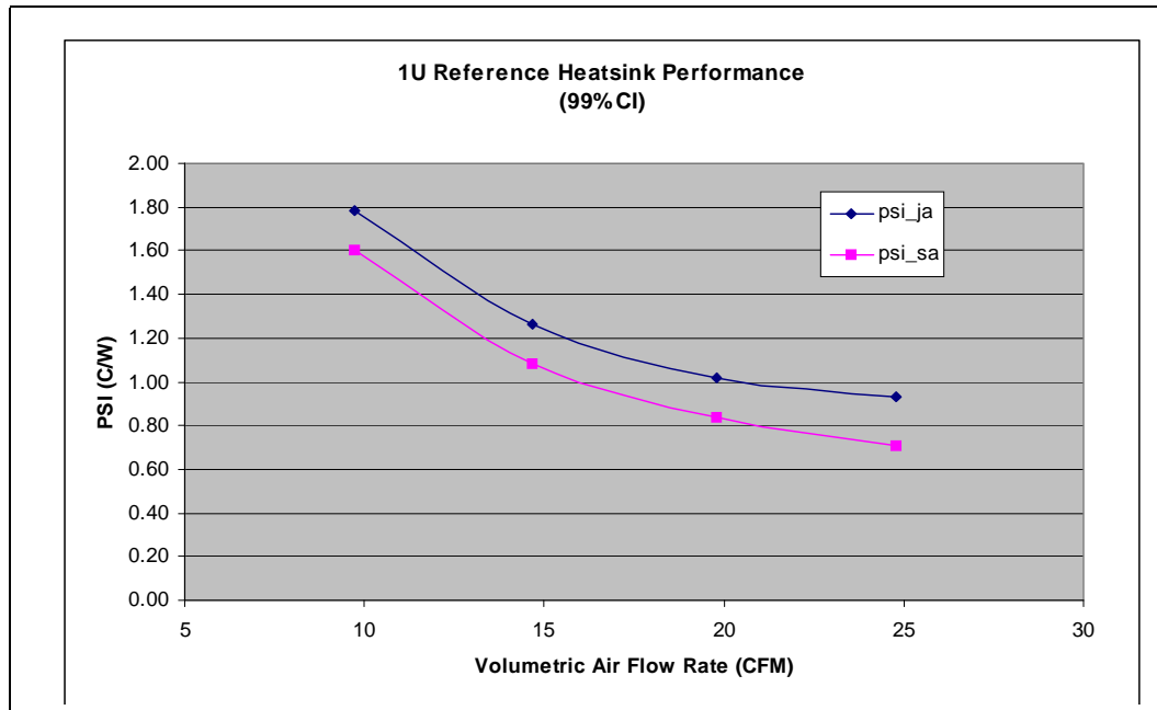
Figure 13. 1U Heatsink Thermal Performance vs. Volumetric Airflow Rate
