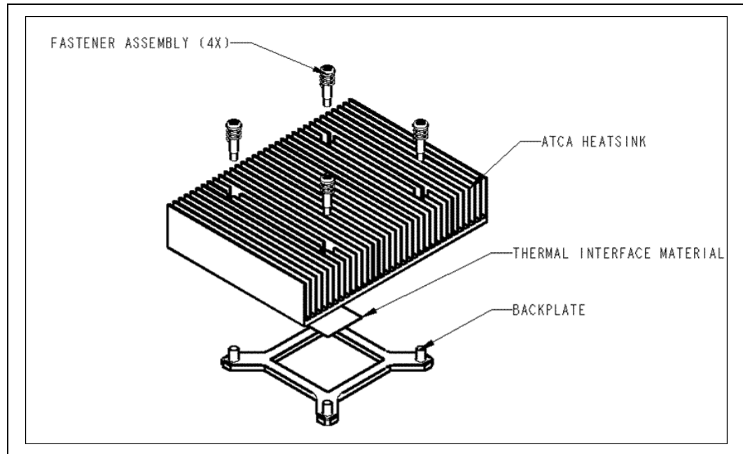
Figure 10. AdvancedTCA* Reference Heatsink Assembly
