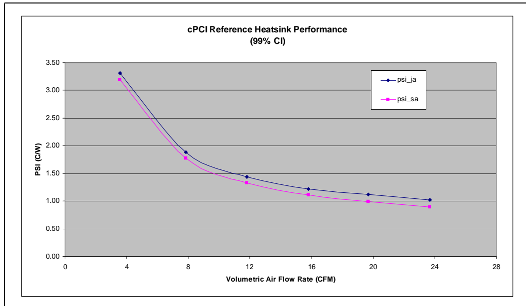
Figure 15. cPCI Reference Heatsink Thermal Performance vs. Volumetric Flow Rate
