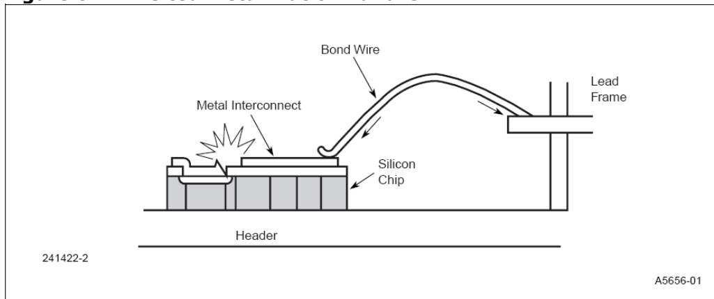
Figure 0-2. Melted Metallization Failure
