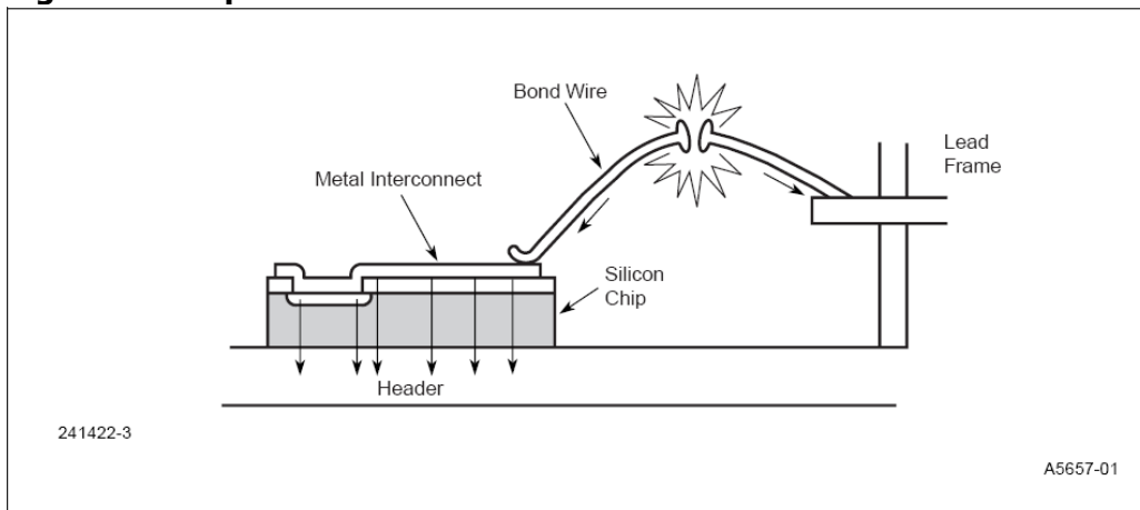
Figure 0-3. Open Bond Wire Failure
