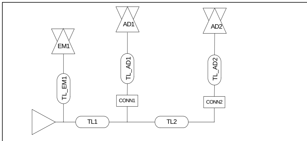
Figure 24. Combination of Slot and Embedded PCI-X 100 MHz Routing Topology
