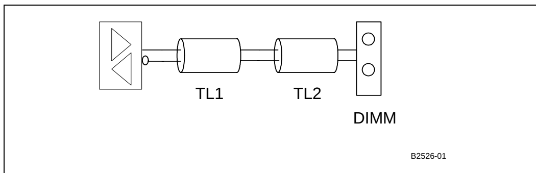
Figure 40. DDR 333 Registered DIMM Clock Topology
