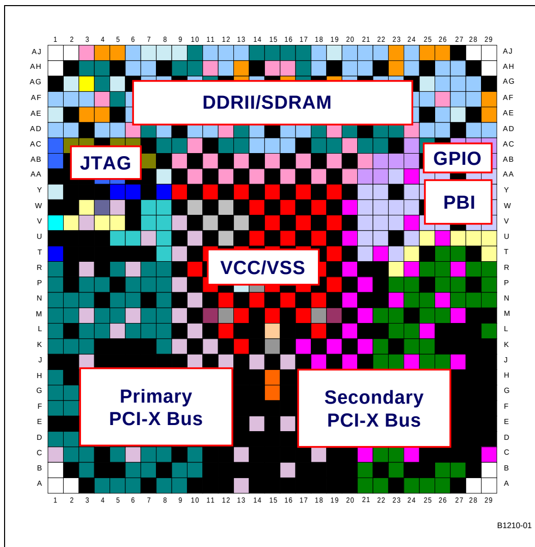
Figure 4. Intel® 80331 I/O Processor Preliminary Ballout (Bottom View)
