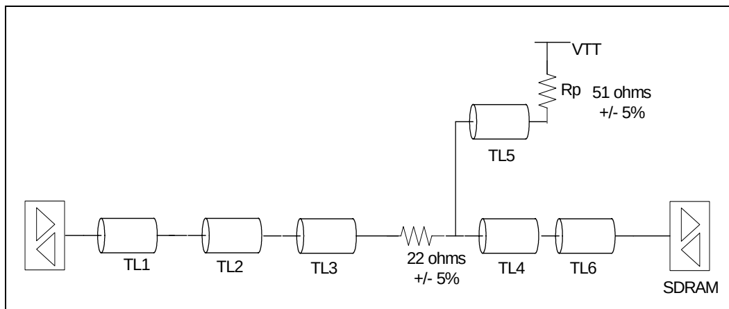
Figure 44. Embedded DDR 333 DQ/DQS Topology
