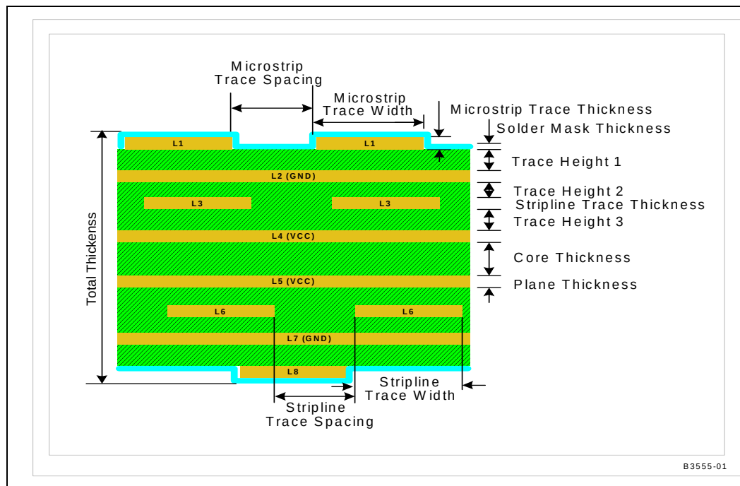
Figure 12. Motherboard Stackup Recommendations
