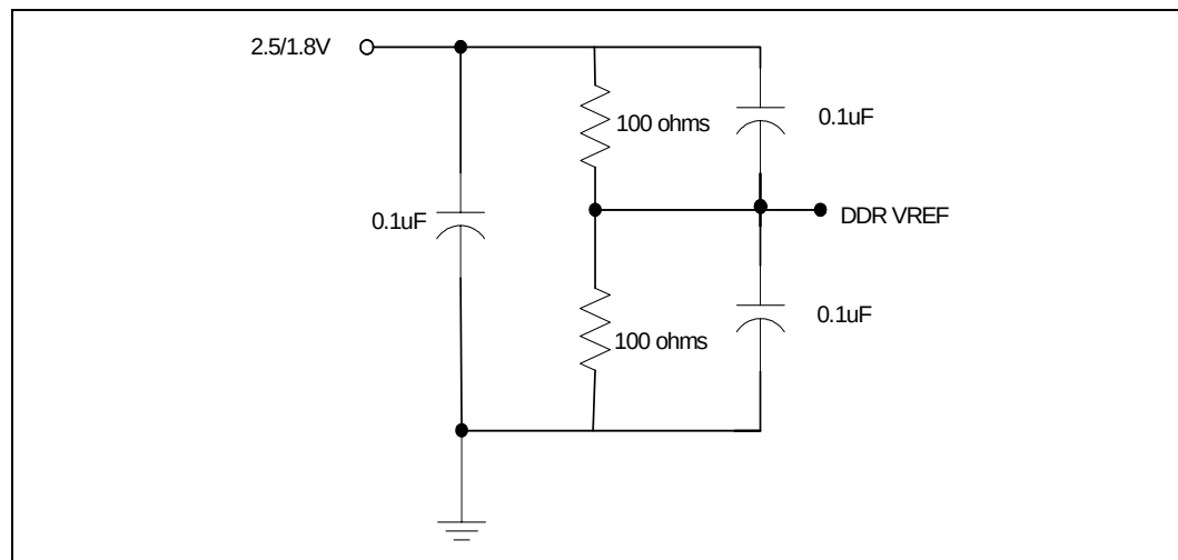
Figure 61. DDR VREF Circuit
