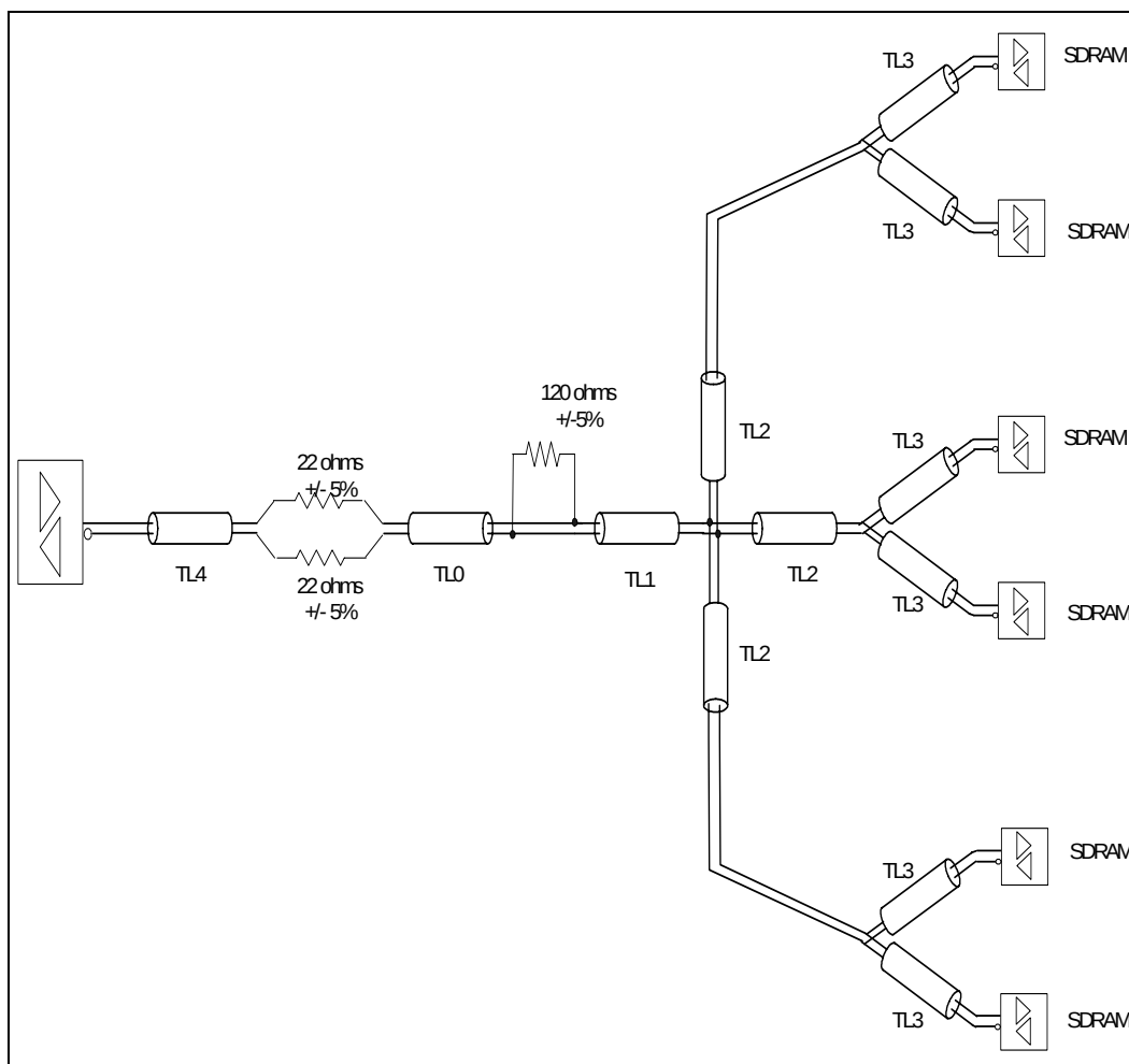
Figure 46. Embedded DDR 333 Unbuffered Clock Topology
