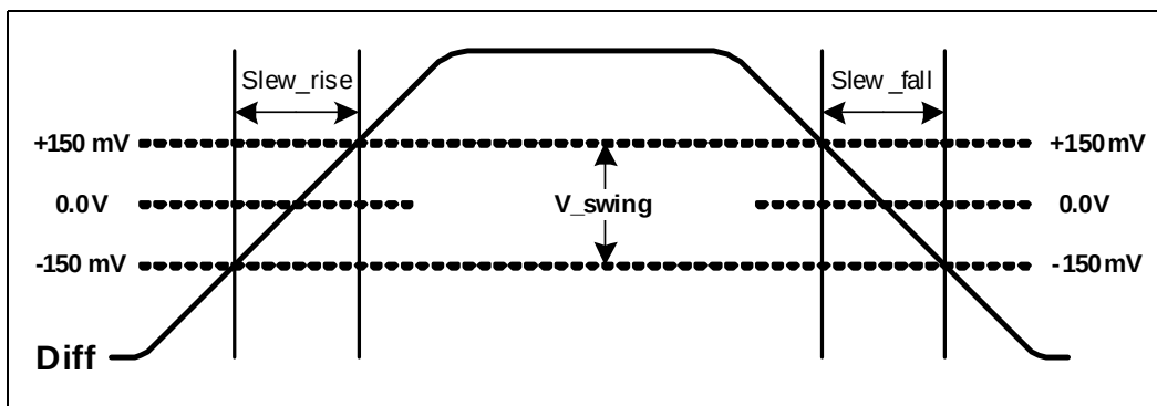
Figure 2-6. Differential Measurements
