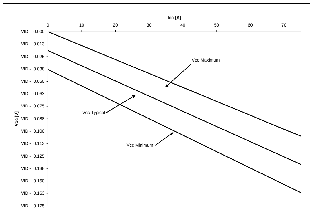
Figure 2-2. V_{CC} Static and Transient Tolerance for Processors with 2 MB L2 Cache
