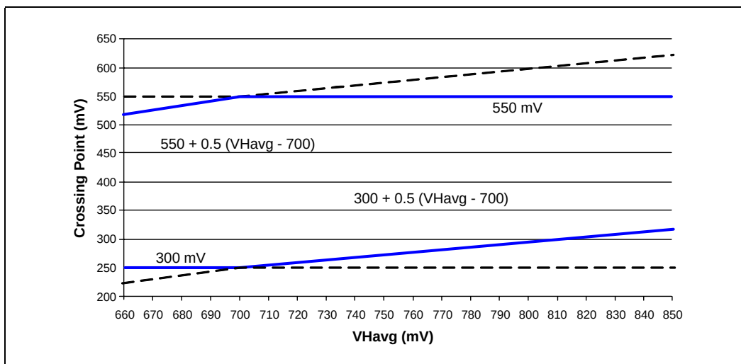
Figure 2-6. Differential Measurements
