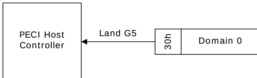
Figure 5-6. Processor PECI Topology
