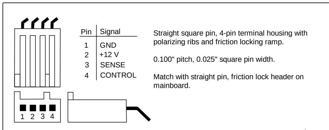
Figure 7-5. Boxed Processor Fan Heatsink Power Cable Connector Description
