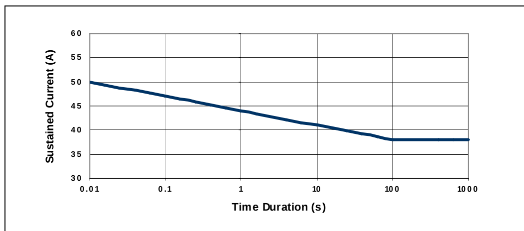
Figure 2-4. Dual-Core Intel® Xeon® Processor L5200 Series Load Current versus Time
