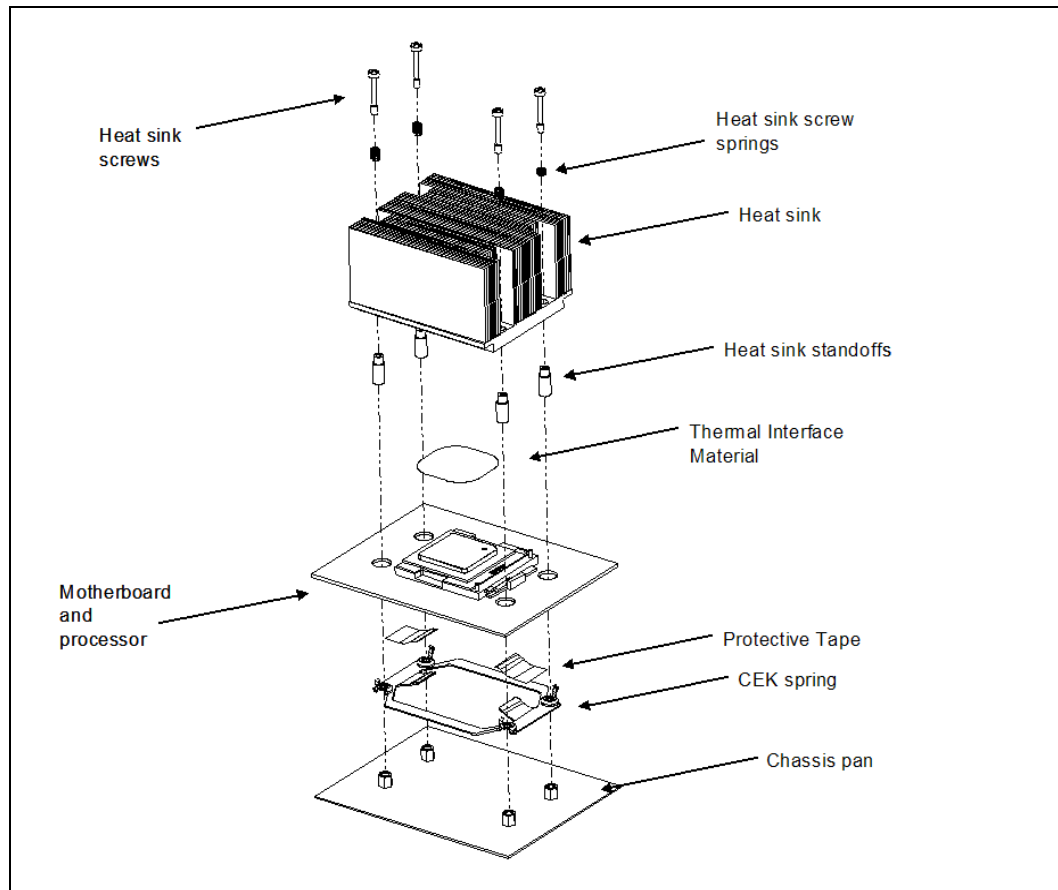
Figure 8-3. 2U Passive Dual-Core Intel® Xeon® Processor 5200 Series Thermal Solution (Exploded View)
