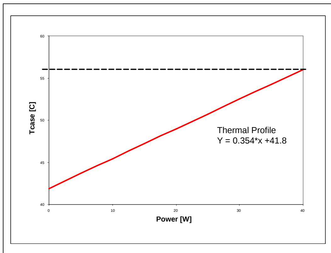
Figure 6-3. Dual-Core Intel® Xeon® Processor L5200 Series Thermal Profile
