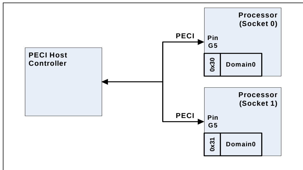
Figure 6-8. Dual-Core Intel® Xeon® Processor 5200 Series PECI Topology
