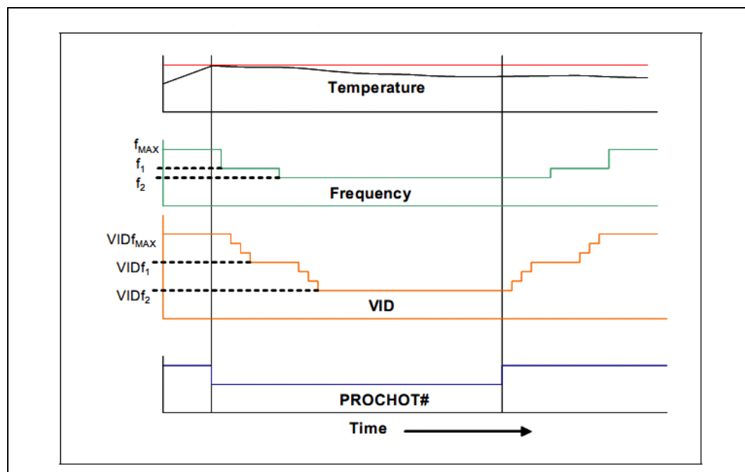
Figure 10. Frequency and Voltage Ordering
