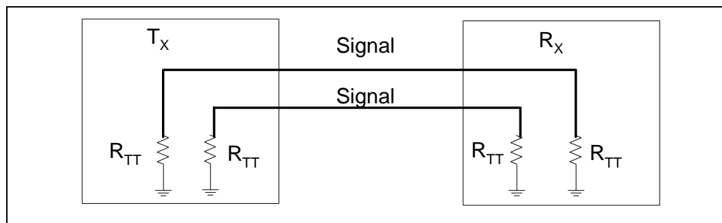
Figure 2-1. Active ODT for a Differential Link Example
