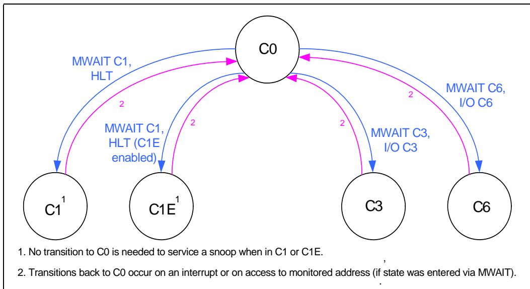
Figure 7-1. Power State
