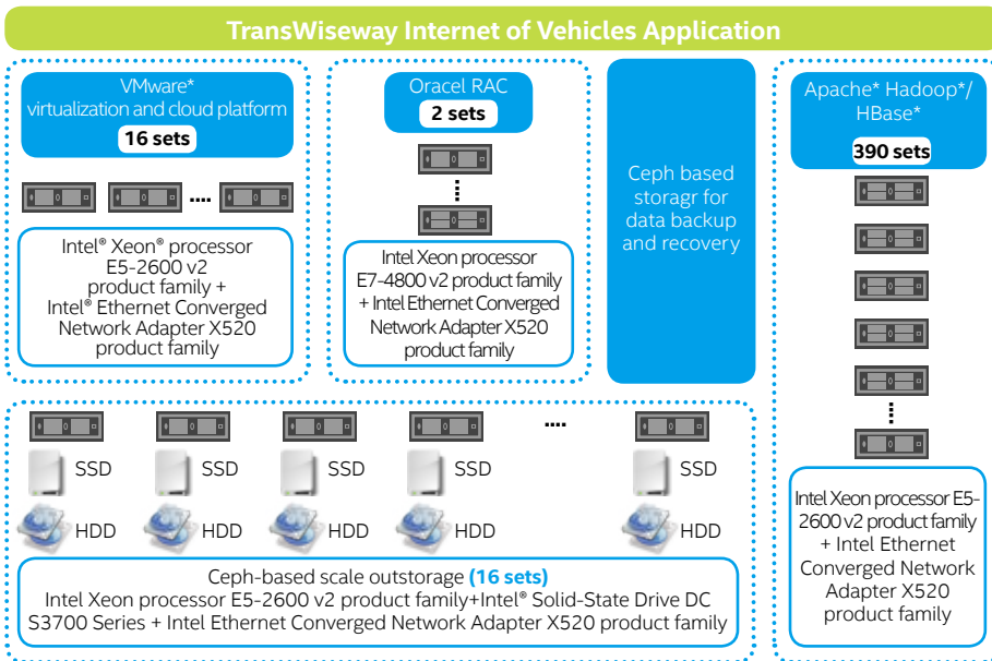
System configuration of TransWiseWay's Internet of Vehicles platform under stress test
