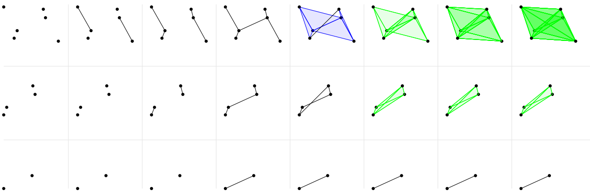
Figure 3: The Vietoris-Rips bi filtration of the heavy atoms of 2,3-butanediol in \mathbb{R}^3 (slightly simplified to save space), using partial charge as the second parameter. Blue is used for triangles and green for tetrahedra. Note the top row is identical to Figure 1, while the lower rows provide new information.
