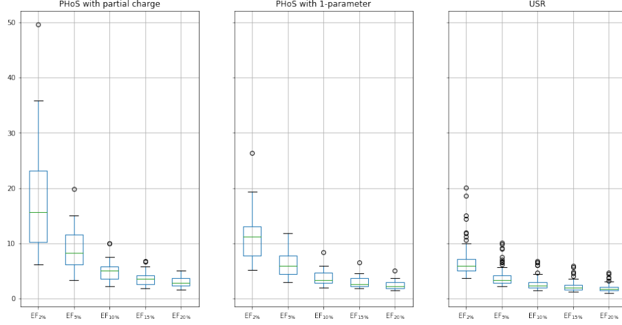
Figure 9: Effectiveness on Cleves and Jain dataset with 1-parameter persistence, 1 conformation, using matching distance. Each column is a box and whisker plot, representing the given EF_\alpha averaged across all queries, with the circles representing outliers. In this plot, we see that 2-parameter persistence with partial charge outperforms both traditional 1-parameter persistence and USR on this dataset.
