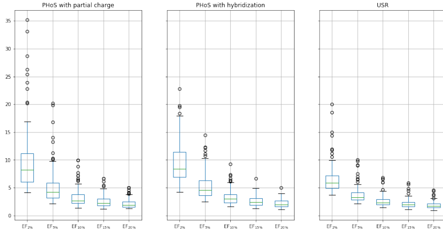
Figure 8: Effectiveness on DUD-E vs. USR, 1 conformation, using matching distance. Each column is a box and whisker plot representing the given EF_\alpha averaged across all queries, with the circles representing outliers. We can see that PH_VS with partial charge and PH_VS with hybridization both greatly outperform USR. The two PH_VS methods perform similarly, with a slight edge to partial charge due to a few high-performing outliers.
