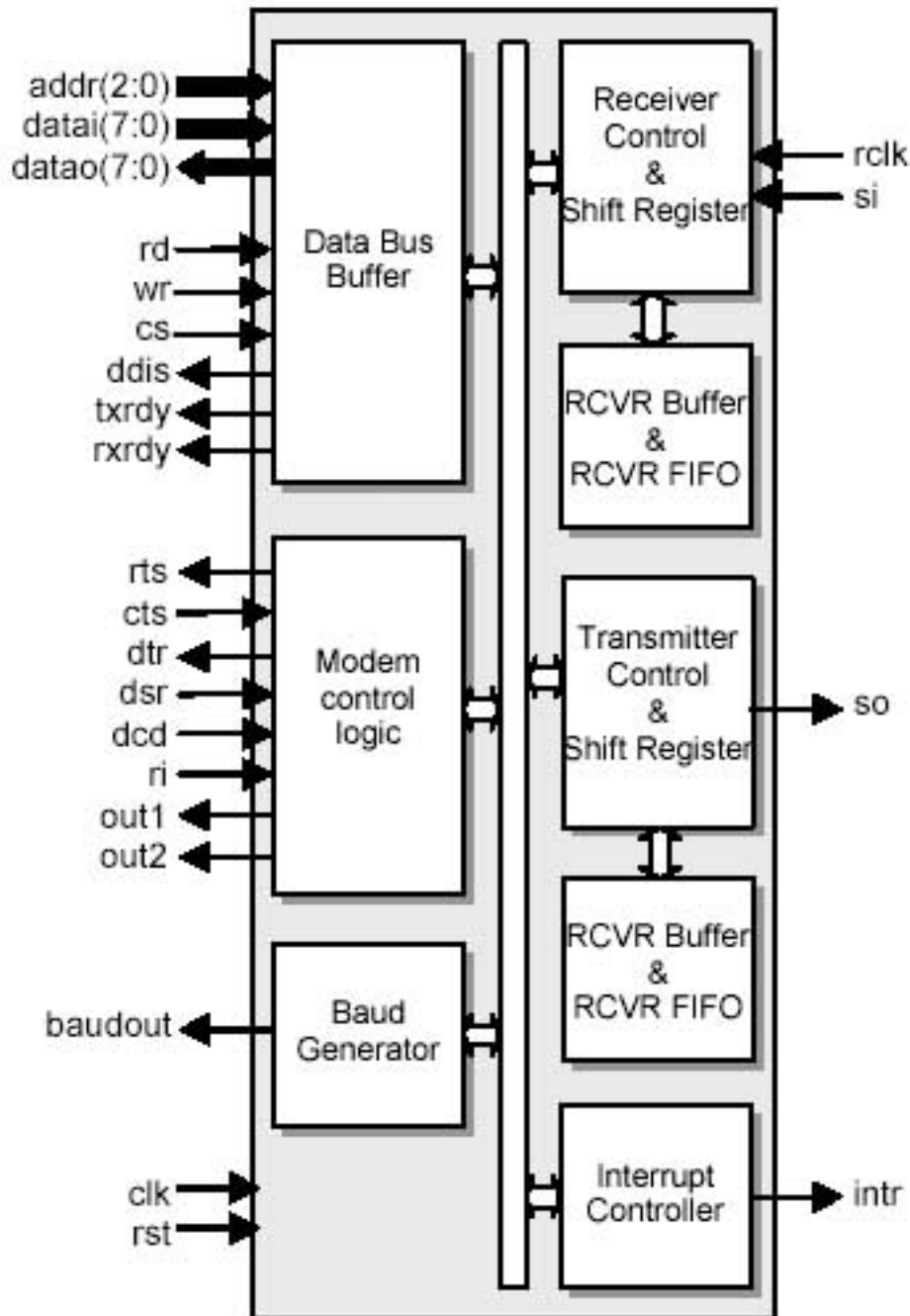
Figure 1. D16550 Block Diagram
