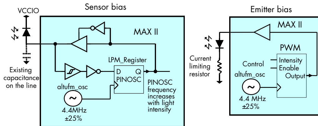
Figure 1. Bias Schematics for Using LED as Sensor and Emitter
