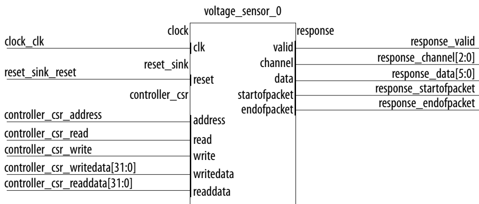
Figure 4. Voltage Sensor Controller with External Sample Storage
