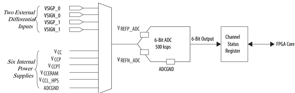
Figure 5. Voltage Sensor
