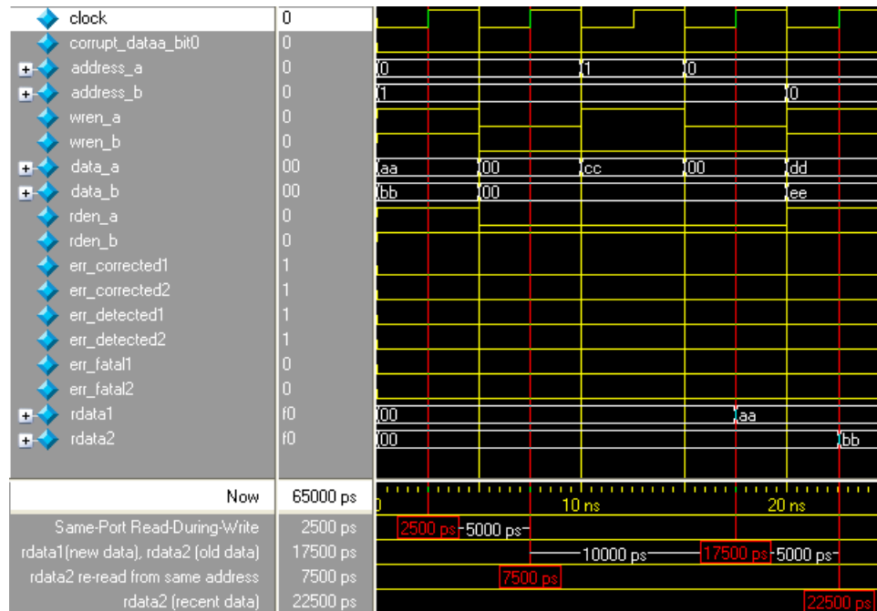
Figure 8. Same-Port Read-During-Write
