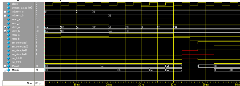
Figure 8. Same-Port Read-During-Write
