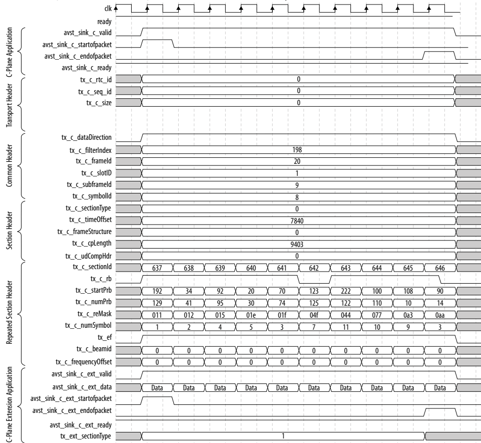
Figure 18. C-plane packet waveform
