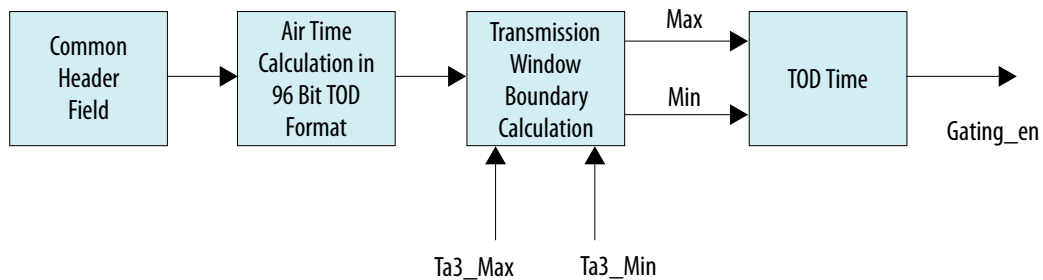
Figure 8. Transmission Window
