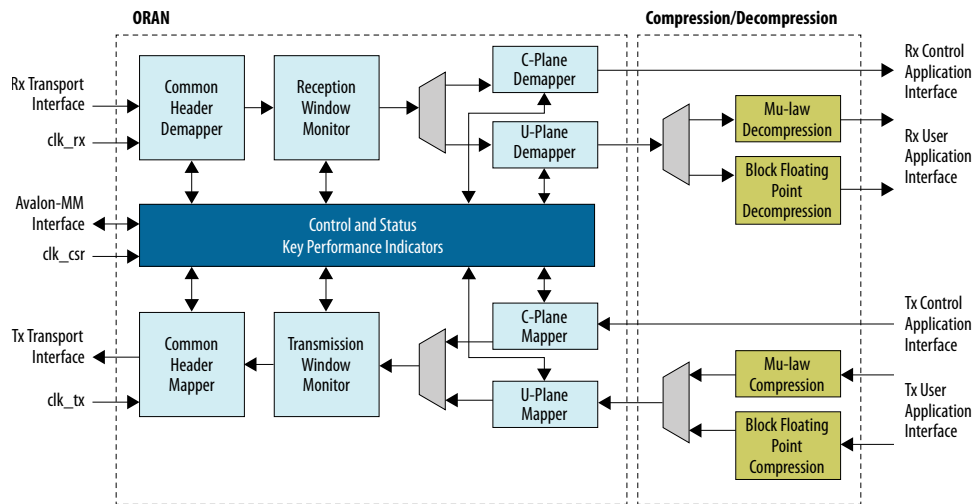
Figure 6. O-RAN IP Block Diagram
