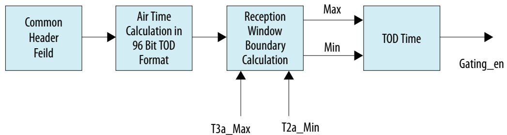
Figure 9. Reception Window
