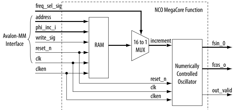
Figure 12. Frequency Hopping Block Diagram
