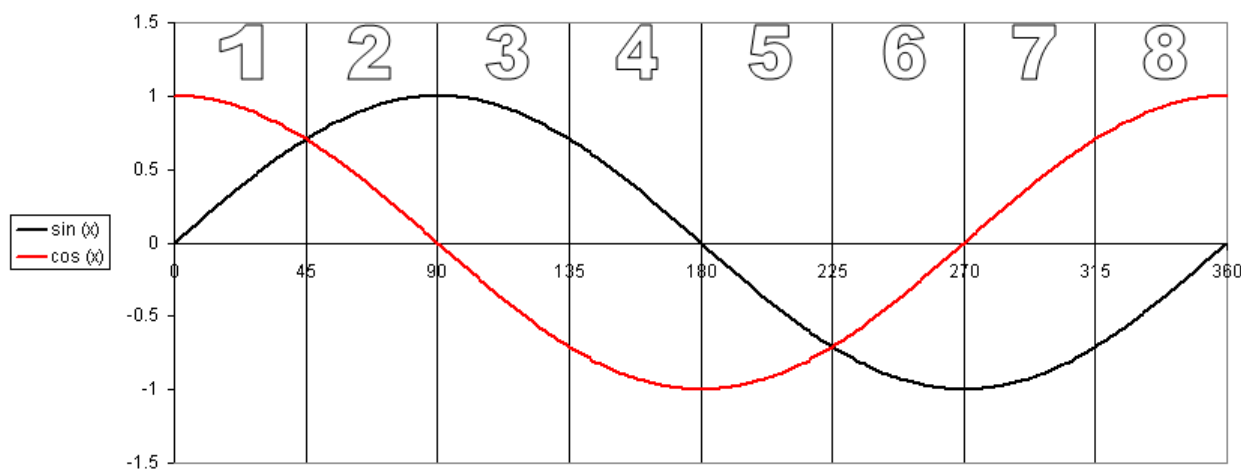
Figure 10. Derivation of output Values
