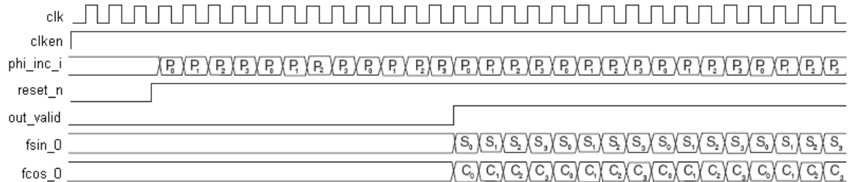
Figure 16. Multi-Channel NCO Timing Diagram with M = 4.
