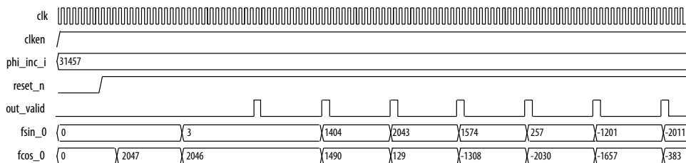
Figure 15. Serial CORDIC Timing Diagram with N = 8
