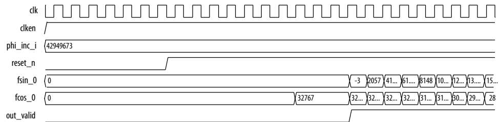
Figure 13. Single-Cycle Per Output Timing Diagram
