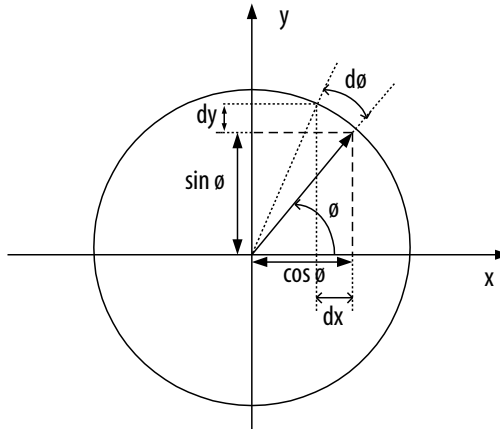
Figure 11. CORDIC Rotation for Sine & Cosine Calculation
