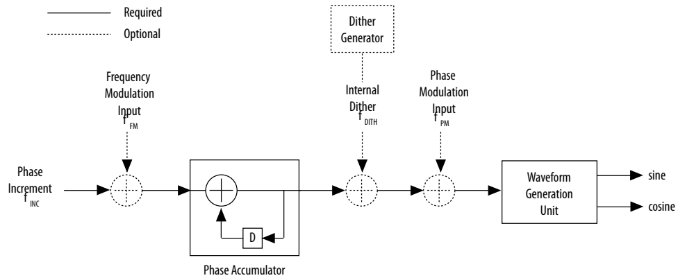
Figure 9. NCO Block Diagram
