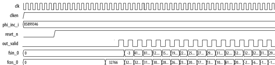
Figure 14. Two-Cycle Multiplier-Based Architecture Timing Diagram
