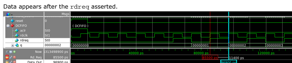
Figure 5. Normal Mode Waveform
