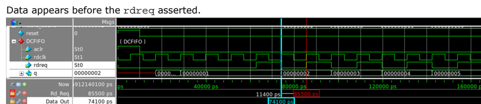
Figure 6. Show-Ahead Mode Waveform
