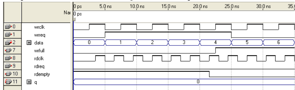
Figure 2. Functional Timing for the wrreq Signal and the wrfull Signal
