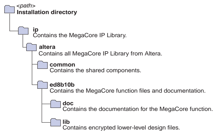
Figure 1-1. Directory Structure
