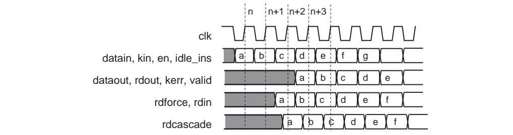
Figure 3-5. Encoder Timing Diagram—Three Cycle Latency
