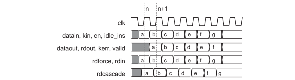
Figure 3-6. Encoder Timing Diagram—One Cycle Latency
