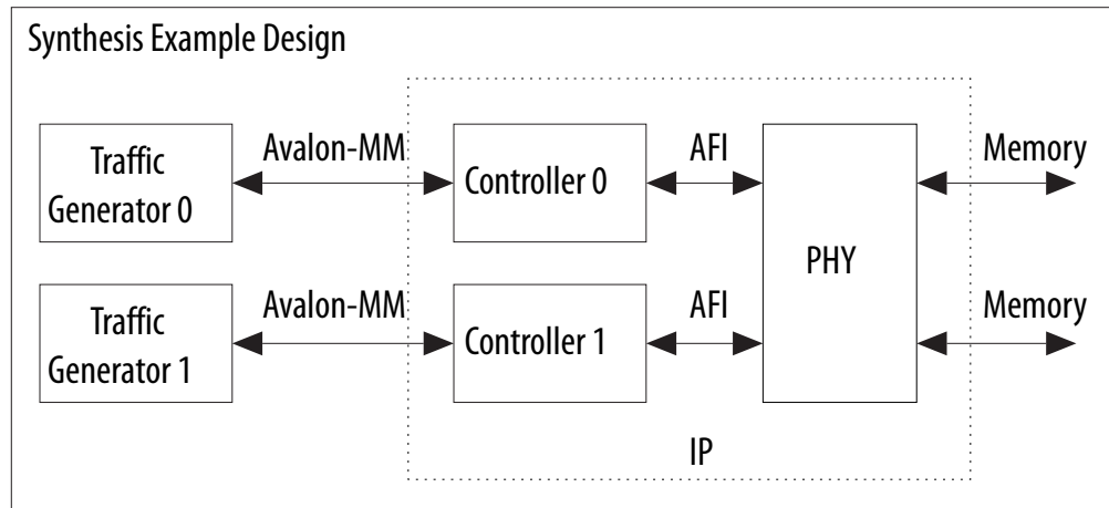
Figure 6. Synthesis Example Design for Ping Pong PHY
