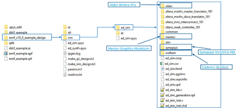
Figure 4. Generated Simulation Design Example File Structure
