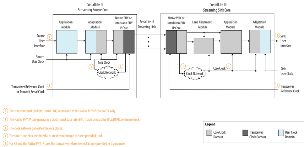
Figure 15. Stratix 10 SerialLite III Streaming IP Core Block Diagram in Standard Clocking Mode
