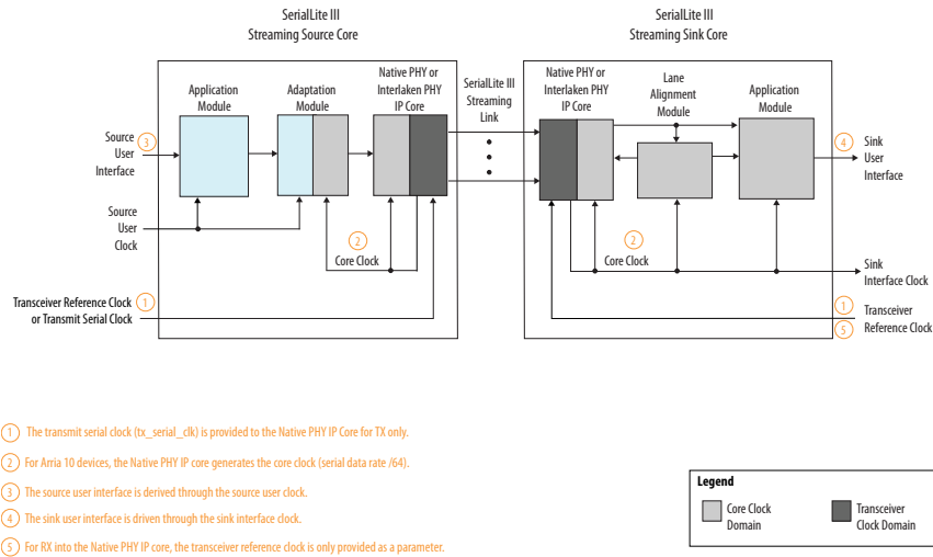
Figure 17. Stratix 10 SerialLite III Streaming IP Core Block Diagram in Advanced Clocking Mode
