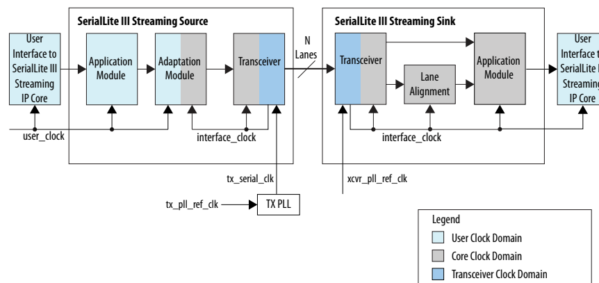
Figure 27. Clocking Structure for Arria 10 Devices
