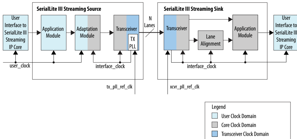
Figure 29. Clocking Structure for Stratix V or Arria V Devices
