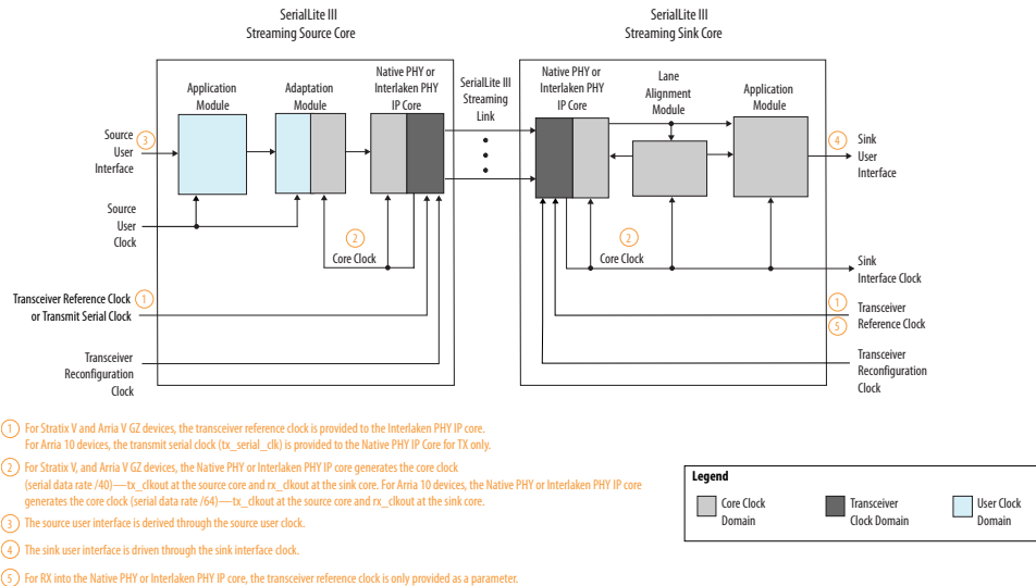
Figure 18. SerialLite III Streaming IP Core Block Diagram in Advanced Clocking Mode
