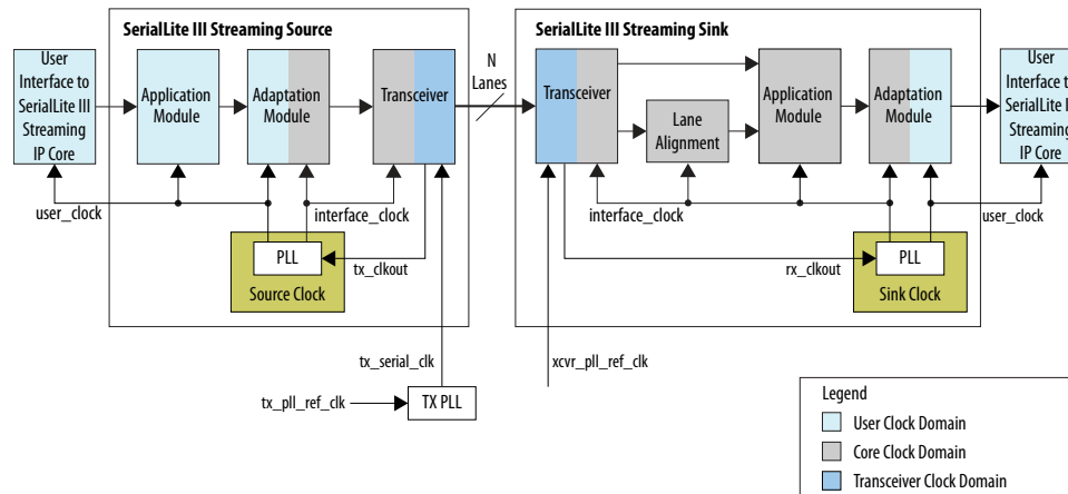
Figure 26. Clocking Structure for Arria 10 Devices
