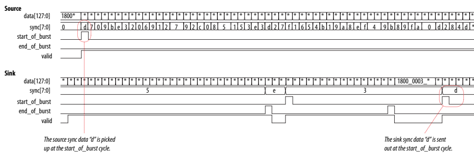
Figure 23. Sink Waveform for Continuous Mode
