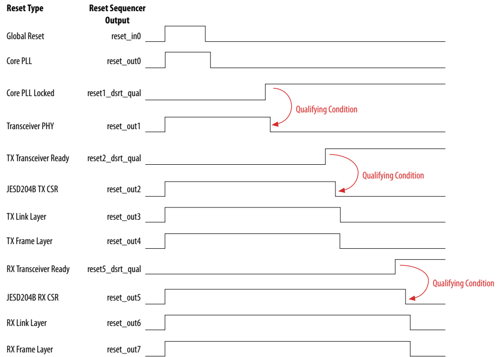
Figure 11. Reset Sequence
