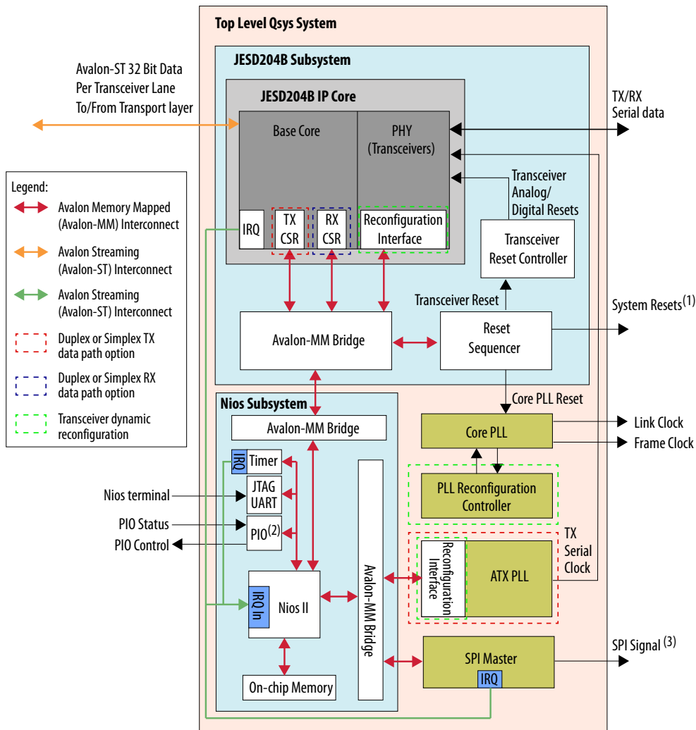
Figure 9. Qsys System for Nios Control Design Example
