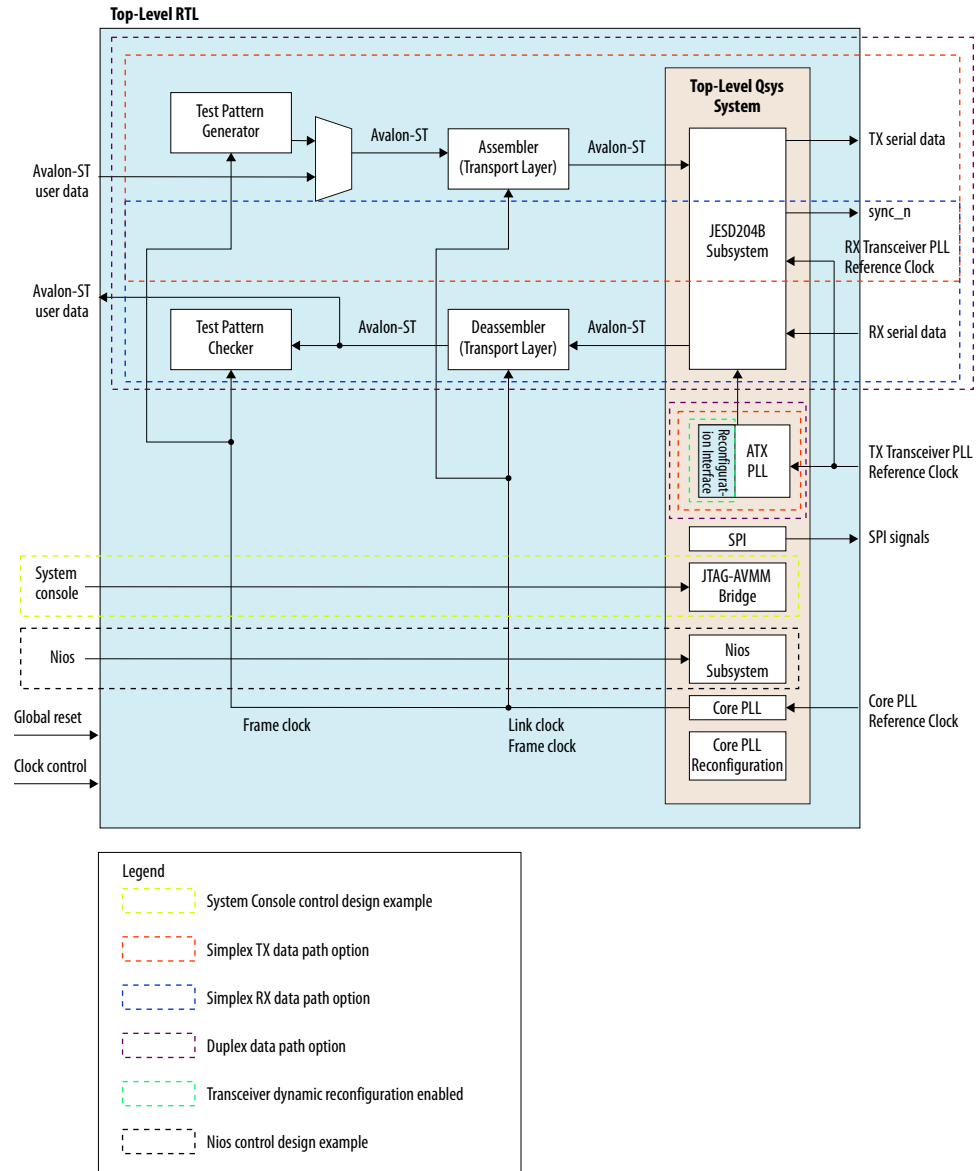
Figure 7. JESD204B Design Example Block Diagram
