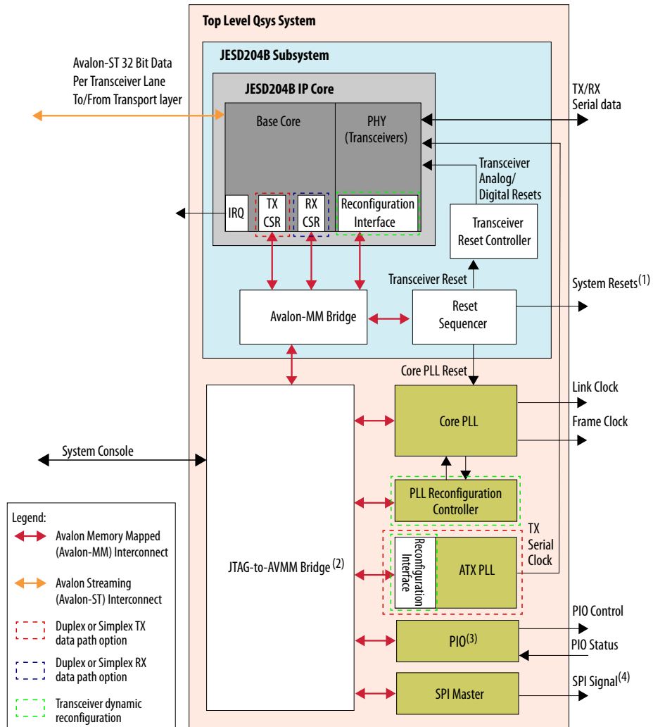
Figure 8. Qsys System for System Console Control Design Example
