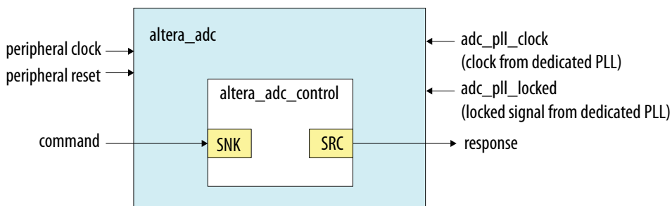
Figure 16. ADC Control Core Only (Modular Dual ADC Core IP Core)
