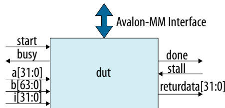
Figure 1. Block Diagram of the Interfaces and Signals for the Component dut
