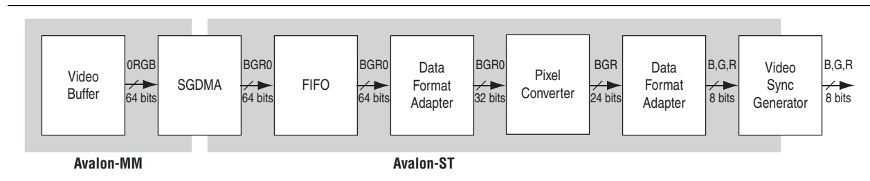
Figure 2. Video Pipeline
