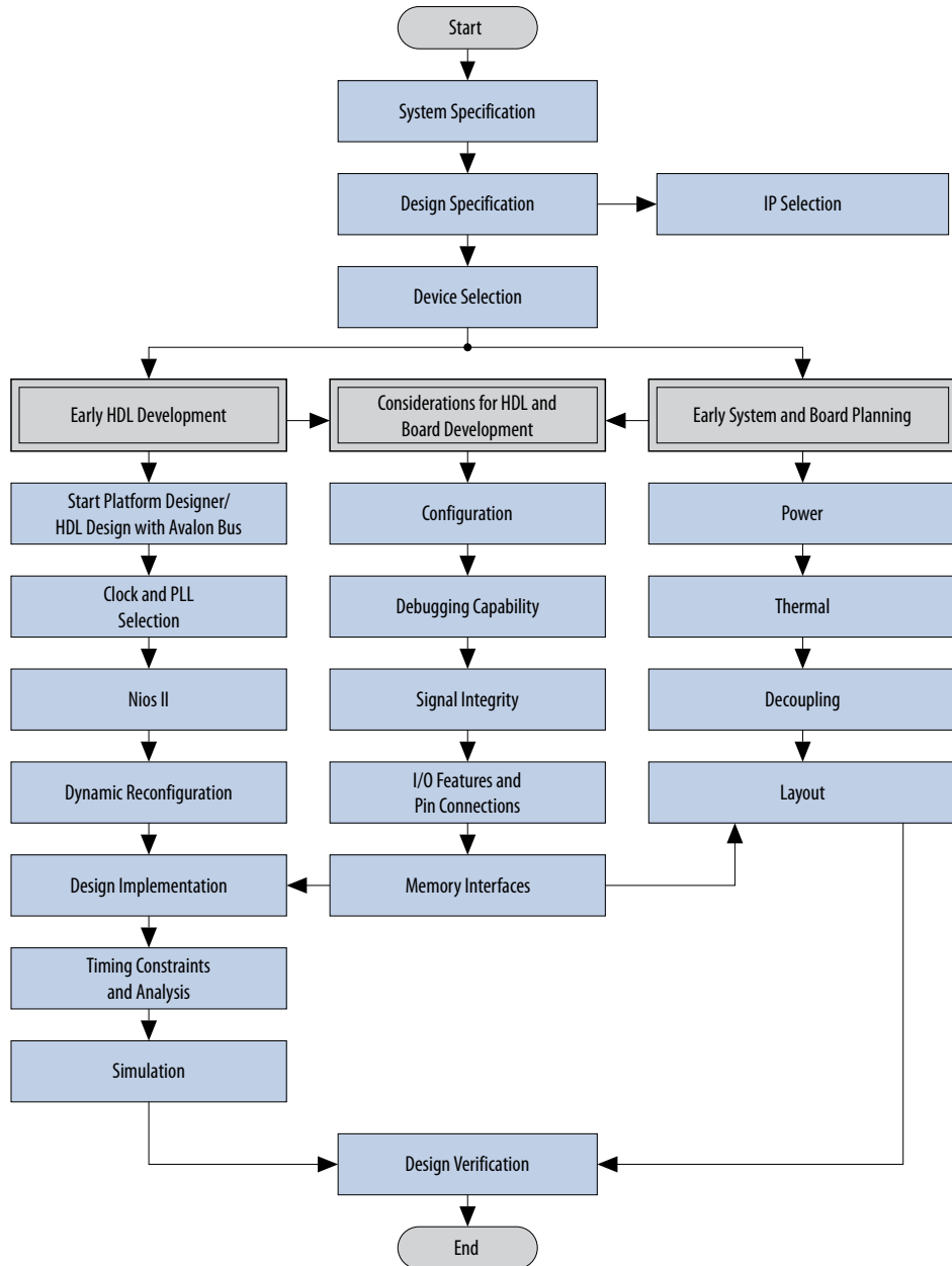
Figure 1. Intel Cyclone 10 LP Device Design Flow
