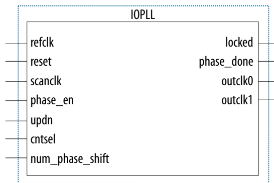
Figure 3. Dynamic Phase Shift Port Ports in the IOPLL IP Core
