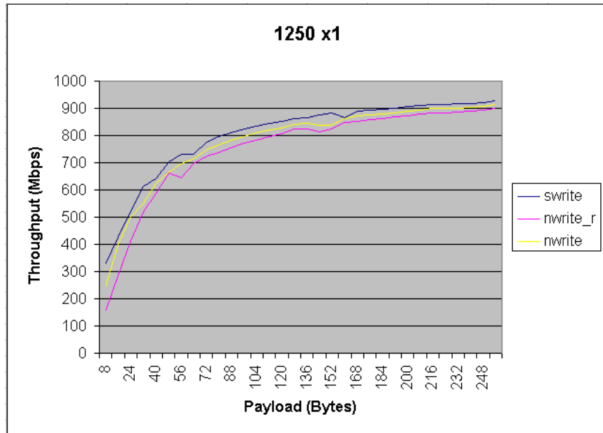
Figure 26. Throughput with Increasing Payload in \times 1 RapidIO MegaCore function at 1.250 Gbaud
