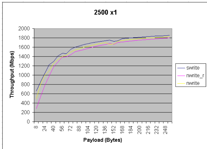
Figure 27. Throughput with Increasing Payload in \times 1 RapidIO MegaCore function at 2.500 Gbaud
