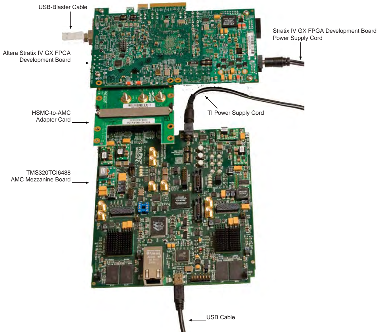
Figure 4. Altera Stratix IV GX FPGA Development Board and Spectrum Digital TMS320TCI6488 AMC Mezzanine Board
