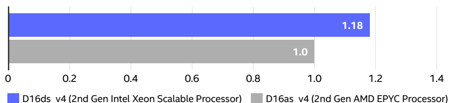
Figure 1. Relative Login Enterprise overall performance of the 16-vCPU Azure Ddsv4 VM and 16-vCPU Azure Dasv4 virtual machines. Higher is better.
