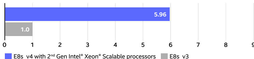
Figure 3. Relative results comparing the ResNet50 benchmark performance of large (64-vCPU) Esv4 VMs vs. Esv3 VMs.
