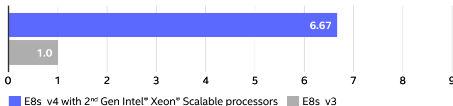
Figure 2. Relative results comparing the ResNet50 benchmark performance of medium (16-vCPU) Esv4 VMs vs. Esv3 VMs.
