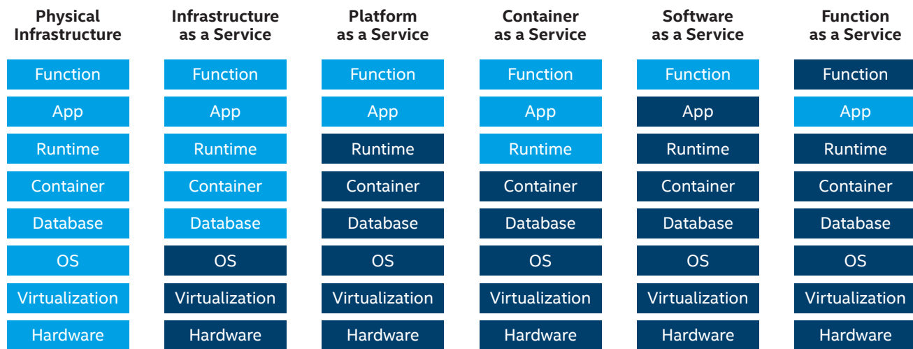
Figure 2. Moving an application up the anything-as-a-service stack abstracts the application from the infrastructure and lets developers concentrate on writing code.
