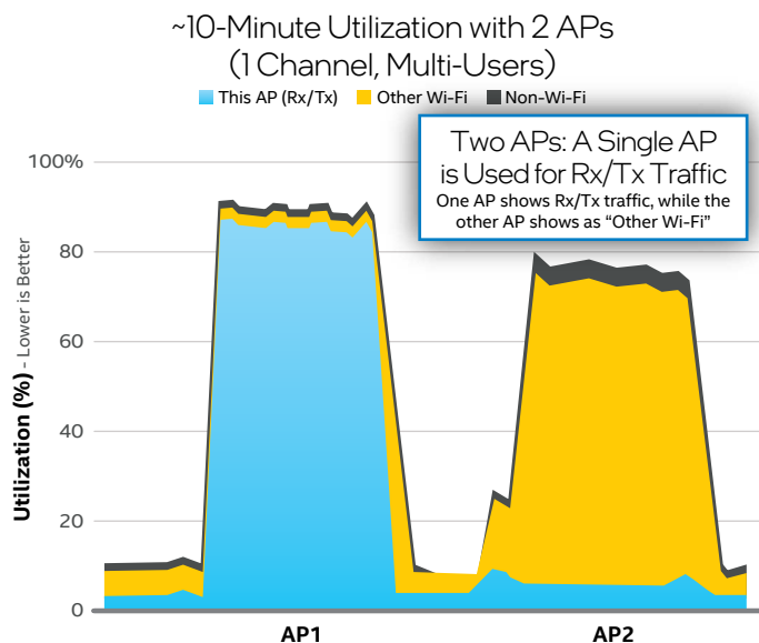
Figure 5. Two neighboring APs operating on the same channel have the same utilization; however, only one AP has users connected and is generating data.
