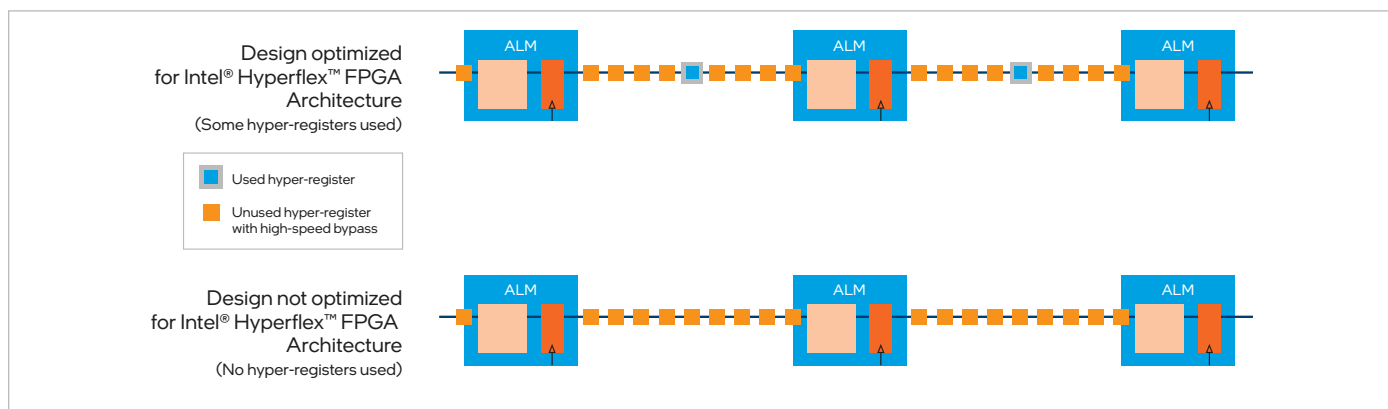
Figure 5. The top design is optimized for Intel® Hyperflex FPGA Architecture; the bottom one is not
