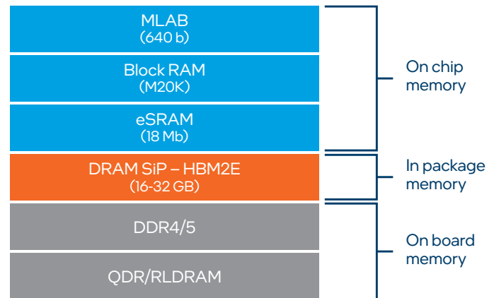
Figure 10. Intel Agilex™ FPGAs support an advanced memory hierarchy—supporting on-chip, in-package, and onboard memory
