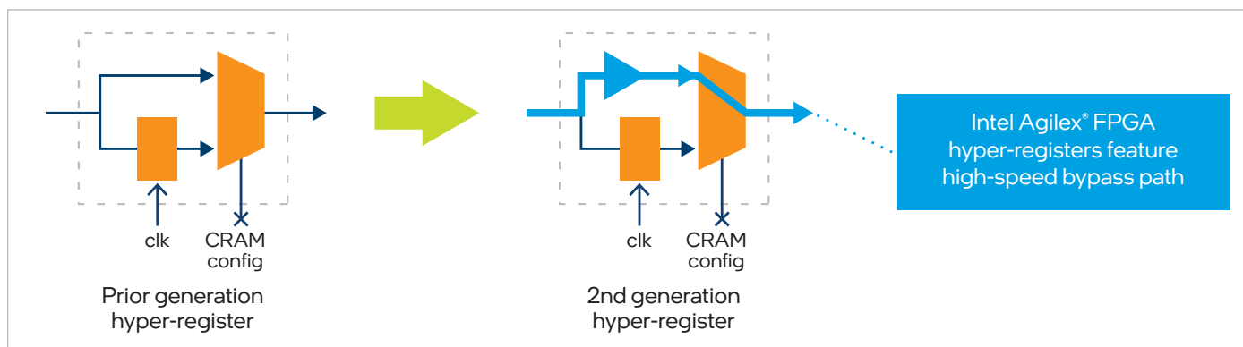
Figure 4. A high-speed bypass accelerates Hyper-Registers to improve fabric performance
