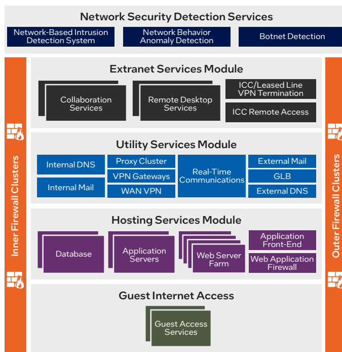
Figure 7. We use enclaves (indicated by the colored boxes), which are networking environments that operate with a common set of security controls, to increase security posture.
