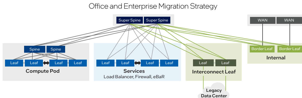
Figure 9. Border router connecting the old topology with the new topology.
