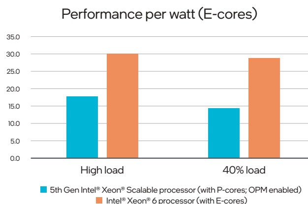
Figure 7. Test results (2)
