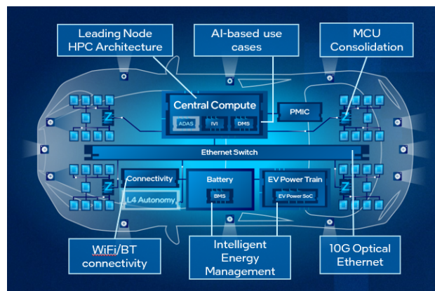
Figure 3 - Future Vehicle Architecture (Domain/Zonal Controllers, Centralized compute)
