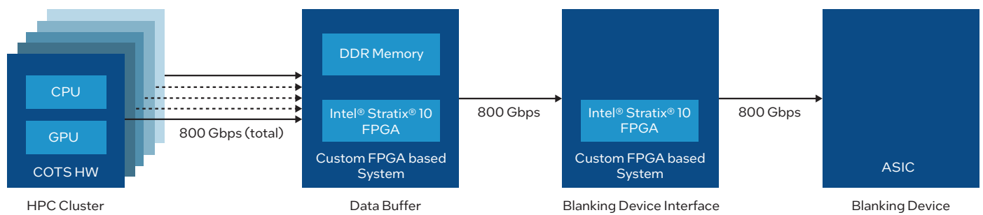
Figure 6. Data Path for IMS MBMW-301 Mask Writer
