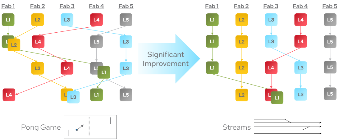
Figure 4. Streamlining materials handling by simulating forward and making better decisions.
