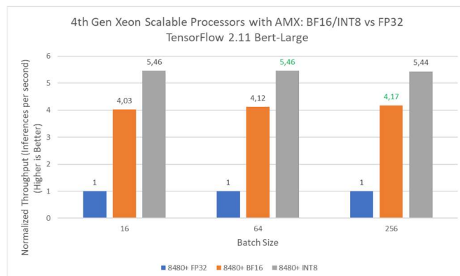
Figure 5. Secured DL Inference Workload Performance for TensorFlow Bert-Large at various at various batch sizes on 4 th gen Intel Xeon Scalable Processors. 5
