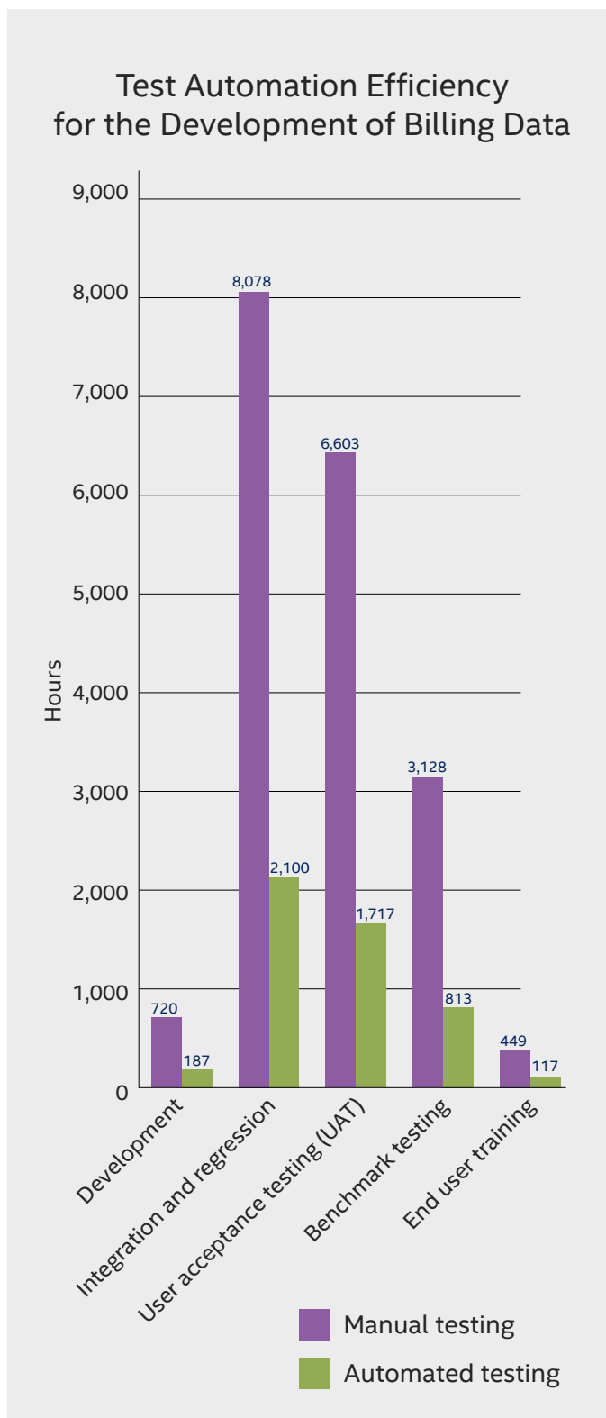
Figure 10. Automating tasks like the development of billing data saved time.
