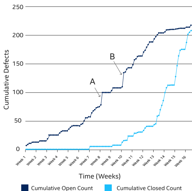
Figure 4. Cumulative open defects trends and cumulative closed defects trends.
