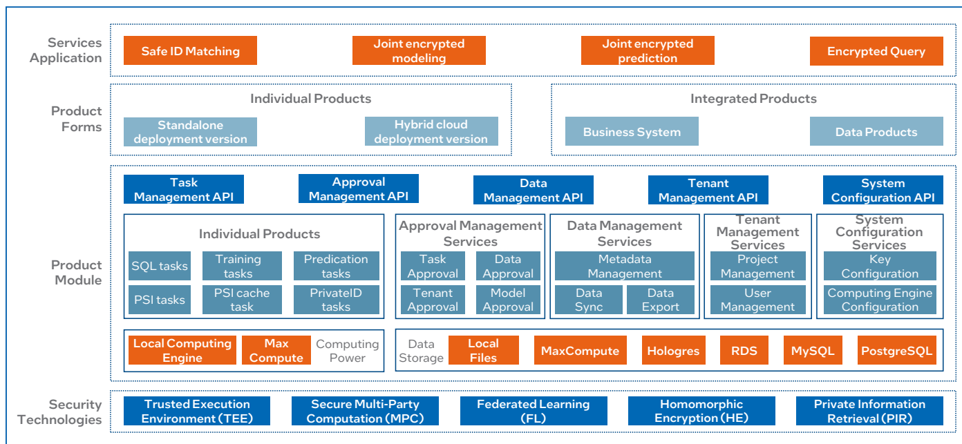
Figure 3. Architecture of Alibaba Cloud DataTrust
