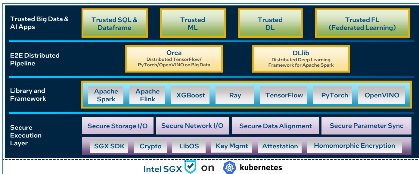
Figure 1. BigDL PPML software stack
